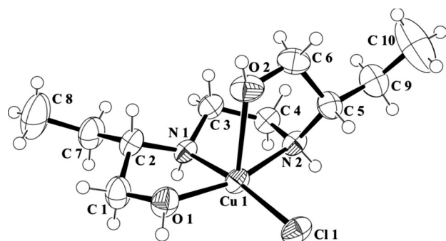
Figure 5. Crystal structure of CuETB complex. Thermal ellipsoids are drawn at the 50% probability level.
