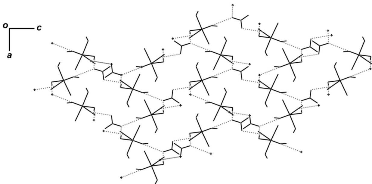
Figure S2. Hydrogen bond design in CuETB crystal structure view along of (A) a axis and (B) b axis. The C atoms were omitted to clarity.
