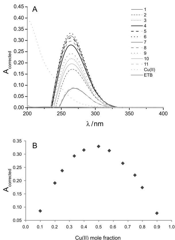
Figure 3. (A) UV-Vis spectra obtained for the continuous variation method; (B) Job's diagram.
