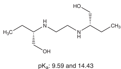
Figure 1. ETB chemical structure.
