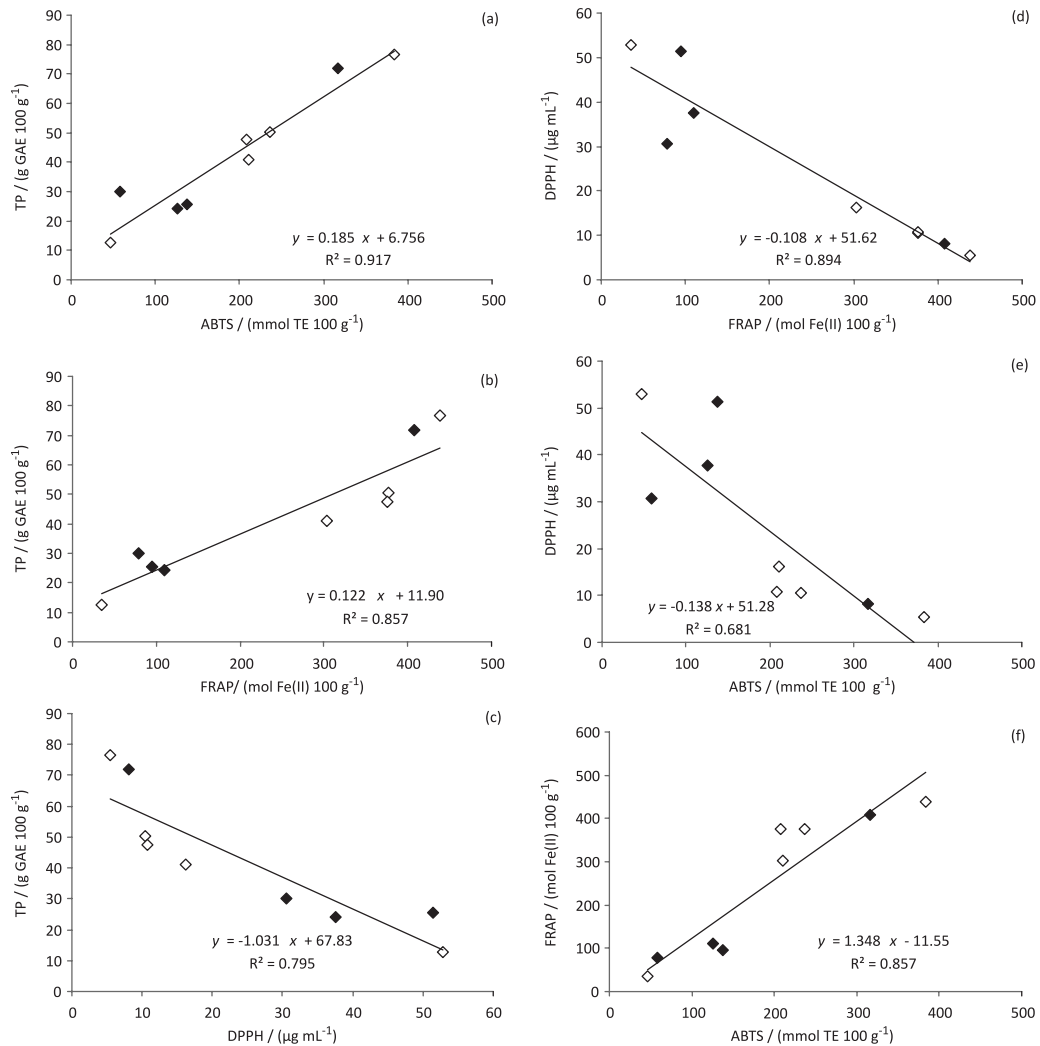
Figure 1. Linear correlations for the extracts between: (a) TP and ABTS, (b) TP and FRAP, (c) TP and DPPH, (d) DPPH and FRAP, (e) DPPH and ABTS, and (f) FRAP and ABTS. White dots: orange blossom honey extracts and black dots: multifloral honey extracts.
