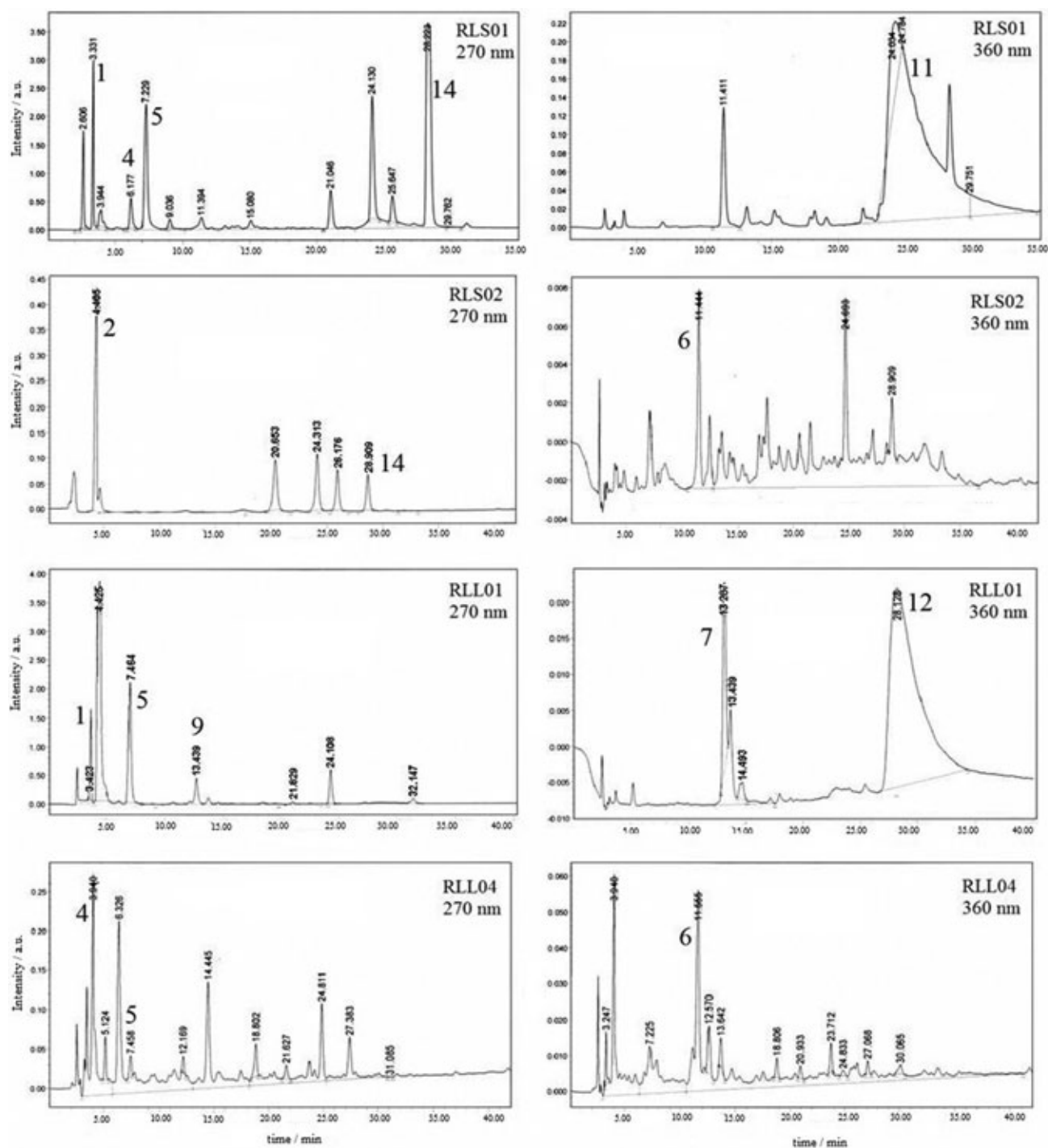
Figure 2. HPLC chromatograms of multifloral and orange blossom honey extracts. For peak identification, see Table 6.
