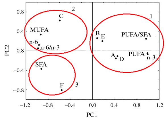
Figure 3. Principal component analysis of the fatty acid composition. PC: principal component; A: experiments 1 to 3; B: experiments 4 to 6; C: experiments 7 to 9; D: experiments 10 to 12; E: experiments 13 to 15; F: experiments 16 to 18 (Soxhlet).
