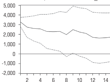
Accumulated Response of D(SUPPRIM_REAL) to D(SUPPRIM_REAL)
