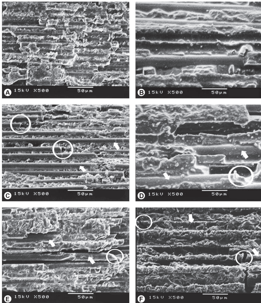
Figure 2. SEM micrographs of the post surfaces after different treatments ( \times 500 ). A: Serrated post treated with 10% HP/10 min. B: Smooth post treated with 10% HP/10 min - slight exposure of the fibers, mostly in smooth posts. C: Serrated post treated with 24% HP/1 min. D: Smooth post treated with 24% HP/1 min - degradation of the resin matrix and exposed fibers (arrows). Discontinuous areas on post surface (circles). E: Serrated post treated with \text{Al}_2\text{O}_3 . F: Smooth post treated with \text{Al}_2\text{O}_3 . Note the exposed fibers (arrows) and discontinuous areas on post surface (circles).
