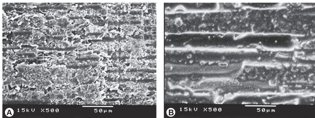
Figure 1. SEM micrographs of the post surfaces with no pretreatment (control) ( \times 500 ). A: serrated post. B: smooth post. Note the continuous fibers and covering the epoxy resin matrix.
