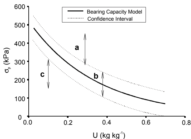
Figure 2 - Criteria used to analyze the effect of harvest operations and wood transport on the preconsolidation pressure of the Typic Acrustox under eucalyptus at 0.10-0.125 m depth.
