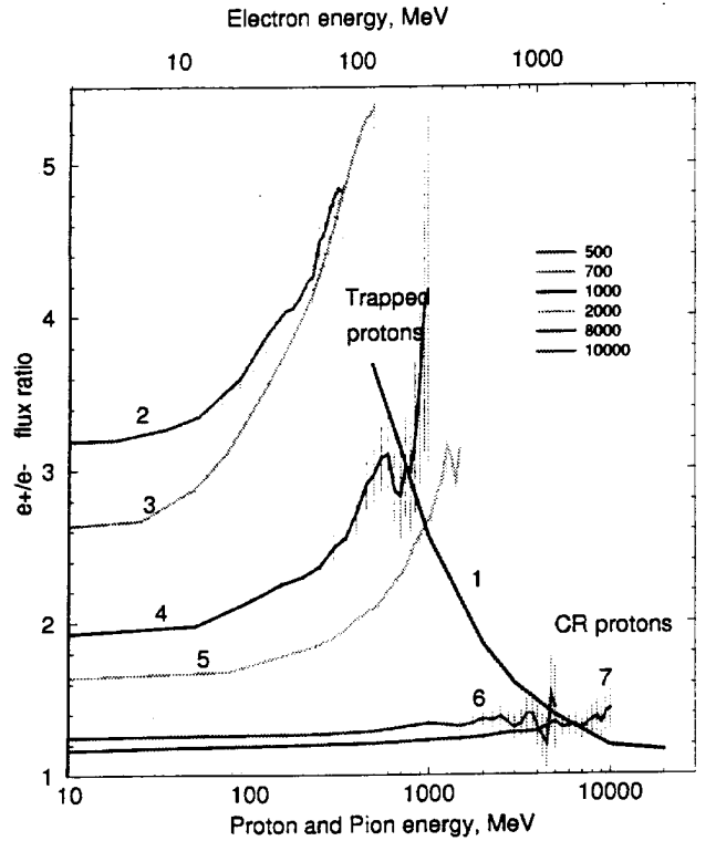
Figure 2. Curve 1: The dependence of the e^+/e^- -flux ratio on the parent proton energy; curves 2 - 7: The dependence of the \pi^+/\pi^- integral production flux ratio and e^+/e^- flux ratio on the \pi and e^\pm energies, correspondingly.
