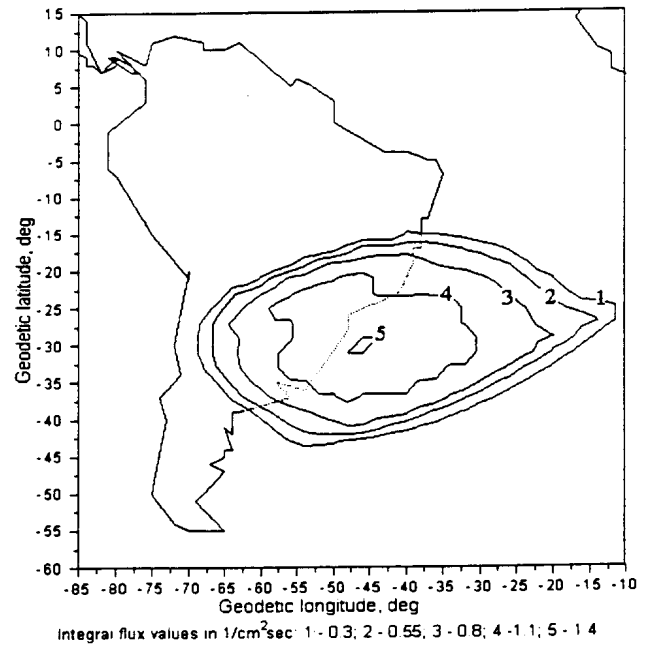
Figure 1. The space distribution of the > 400 \text{ MeV} trapped protons at the altitudes of 400 km according to AP-8 model (Vette, 1991).
