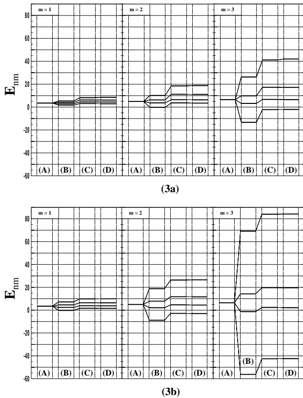
Figure 3a. Some of energy levels for a j = 3/2 system with n = 2 and m = 1, 2 and 3 , as each component of the total Hamiltonian \hat{H} is progressively added, a process that is represented by columns (A), (B), (C), and (D). Figure (3b) is the radiation intensity-dependent version of Figure (3a).
