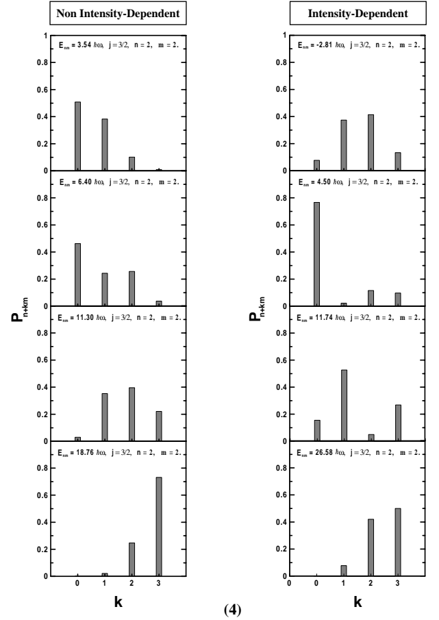
Figure 4. Weight of each component, P_{n+km} = C_{n+km}^2 , in the composition of the state vectors, |\Psi_{nm}^{(1,2,3,4)}\rangle for j = 3/2 , and n = m = 2 . The left column is for a non intensity-dependent interaction and the right column is for an intensity-dependent one.
