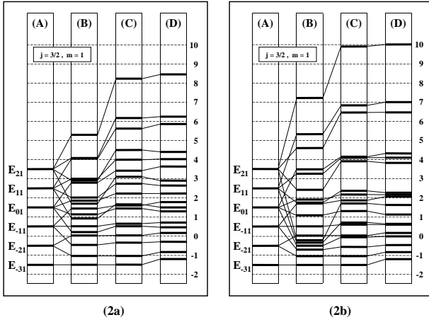
Figure 2a. The j = 3/2 version of Figs. (1a) and (1b).
