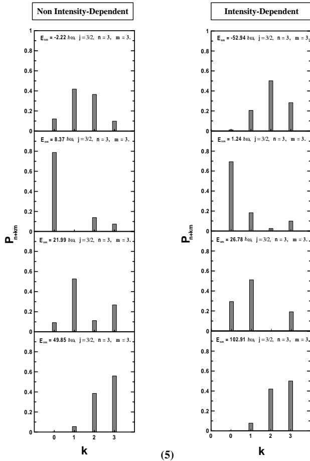
Figure 5. The version of Fig. (4) for n = m = 3 .
