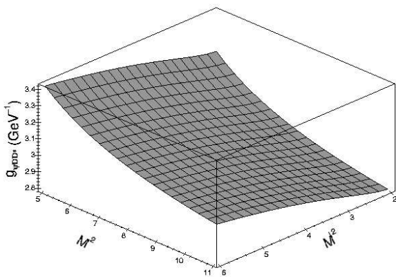
Figure 3. M^2 and M'^2 dependence of g_{\psi DD^*}^{(D)}(Q^2 = -0.21 \text{ GeV}^2) .
