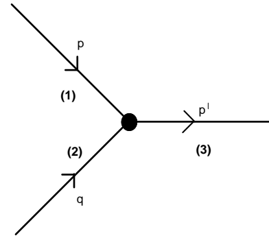
Figure 1. Diagram representing the H_1(p)H_2(q)H_3(p') vertex.
