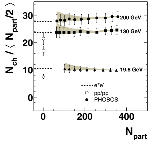
Figure 2. \langle N_{ch} \rangle / \langle N_{part} \rangle vs. N_{part} for \sqrt{s_{NN}} = 19.6, 130, and 200 GeV (closed symbols). The error includes contributions from the uncertainty on overall N_{ch} scale and N_{part} scale. The shaded band shows the uncertainty on the extrapolation procedure for larger \eta . The open symbols show UA1 p \bar{p} data at 200 GeV and interpolated results for the lower energies. The dotted lines show the values for e^+e^- .
