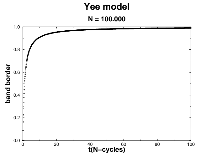
Figure 17. Yee model.
