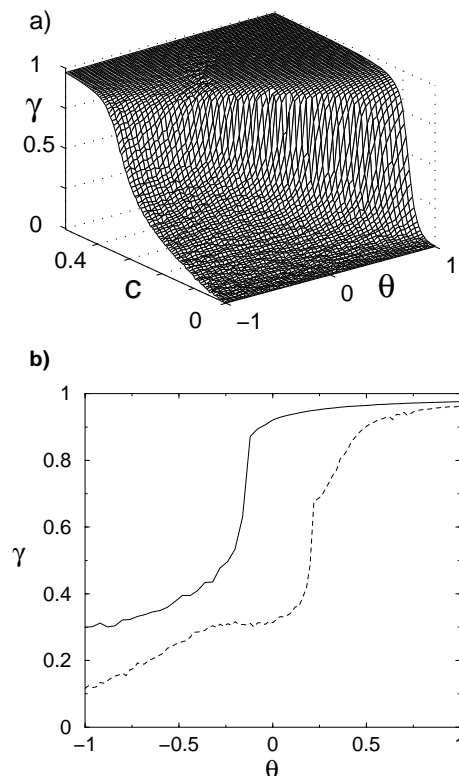
Figure 3. a) Pearson's coefficient \gamma (see text for definition) vs. the parameter space ( c, \theta ). Other parameters are \alpha = 2 , \beta_1 = -0.95 and \beta_2 = -1.2 (case PT-AT(II)). b) Solid line: \gamma vs. \theta [cut of the \gamma -surface in a)] at c = 0.25 , highlighting the role of asymmetry in enhancing synchronization. The dashed line reports the same for the PT-AT(I) case already studied in Ref. [16].
