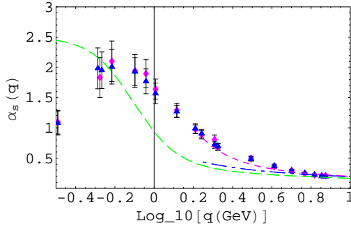
FIG. 3: The running coupling \alpha_s(q) as a function of \log_{10} q(\text{GeV}) of MILC c ( a = 0.12\text{fm} ) \beta_{imp} = 6.76 (triangles) and 6.83 (diamonds), (50 samples each).
