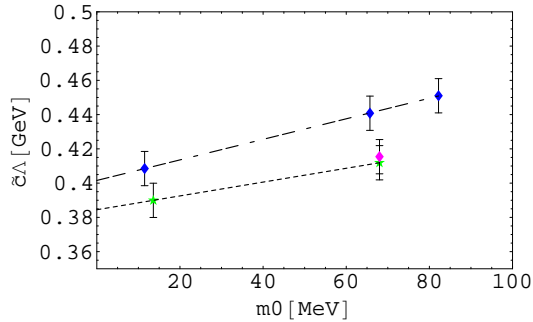
FIG. 6: The chiral symmetry breaking mass \tilde{c}\Lambda as a function of bare mass and its chiral limit. Dotted line is the extrapolation of MILC_f, \beta_{imp} = 7.09 and the dash-dotted line is that of MILC_c, \text{Asqtad} action.
