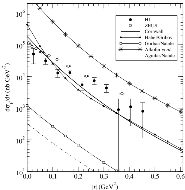
FIG. 4: \rho photo-production differential cross section, compared with the H1 and ZEUS data [18, 19]
