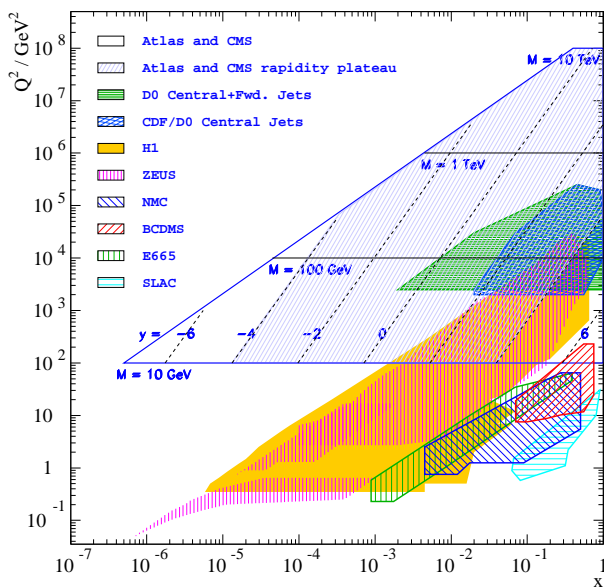
FIG. 1: Kinematic coverage of the DIS and collider pp and p\bar{p} experiments. For pp and p\bar{p} colliders, the Bjorken x_1 and x_2 of the interacting quarks are related to the mass M of the Drell-Yan pair and its rapidity y as x_{1,2} = M/\sqrt{S} \exp(\pm y) where S is the center of mass energy squared for the experiment.
