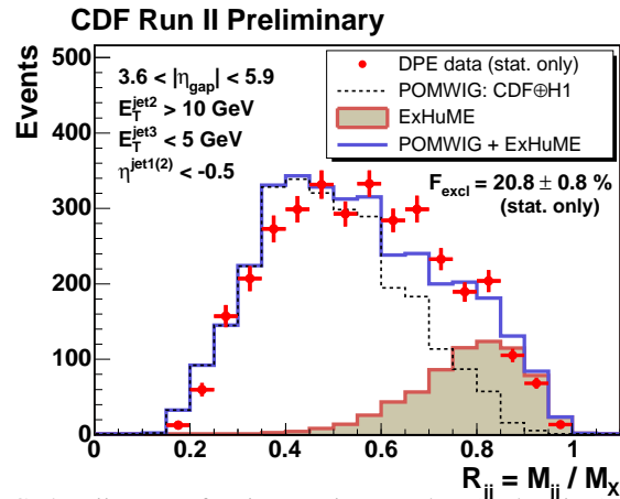
FIG. 4: Dijet mass fraction R_{jj} in DPE data (dark points) and best fit (solid line) obtained using inclusive (dashed line) and exclusive ExHuME (shaded line) MC predictions.
