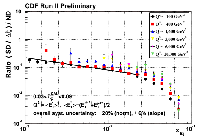
FIG. 1: Ratio of SD to ND event rates as a function of x_{Bj} for different Q^2 ranges. Data sample of 128 pb -1 .
