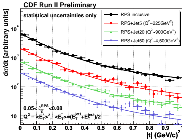
FIG. 2: t distributions in soft and hard SD events for different Q^2 ranges.
