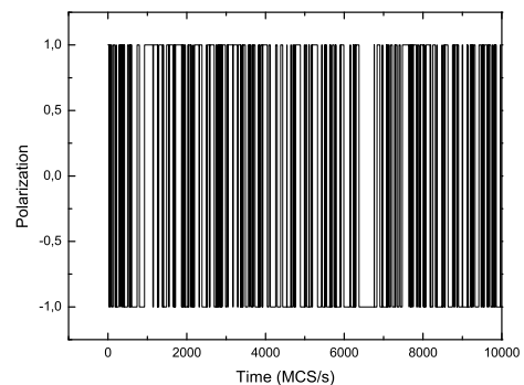
FIG. 7: A binary version of the dependence in Fig. 2b. It was assigned a value 1 to all values M > 0 and a value of -1 for all values M < 0 . Note the similarity with Fig. 1 where actual reversals are presented.
