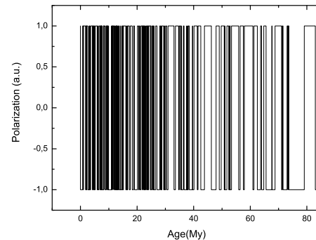
FIG. 1: Representation of geomagnetic reversals from around 80 My ago to our days. We arbitrarily have assumed -1 as the current polarization. We have not plotted the period from 80 My to 165 My (for which also a record exists) for the sake of clarity. There was a period with no reversals from 80 to 120 My (the beginning appears in the plot). The period from 120 My to 165 My was very similar to the period from 0 to 40 My (in number of reversals and in the average duration of reversals). The data was obtained from Cande and Kent [8,9].
