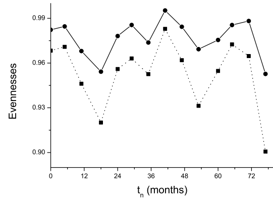
FIG. 3: Evenness indices E_{q^*} (dotted line) and E_1 (solid line) versus t_n for the dataset described in Table I.
