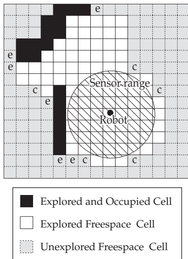
Figure 1. Region of the environment where the BVP is calculated. Searching for edges of walls, regions labeled as e, represents a wall-following exploring behavior and for unexplored concave regions, labeled as c, it corresponds to a space-filling exploring behavior.
