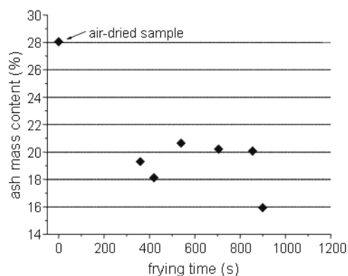
Figure 7: Ash content of the sludge samples fried for different lengths of times. T_{\text{oil}} = 180^{\circ}\text{C} .
