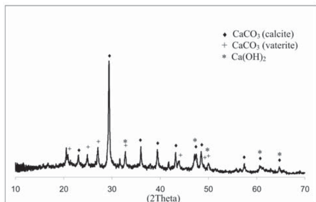
Figure 2: X-ray diffraction pattern showing the main compounds present in the textile residue as received from the textile industry. [Figura 2: Difratoograma de raios X mostrando os principais compostos presentes no resíduo têxtil bruto.]
