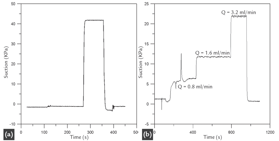
Figure 4 Preliminary results: a) B Parameter test results; b) Constant flow rate test results to obtain k_{sat} .
