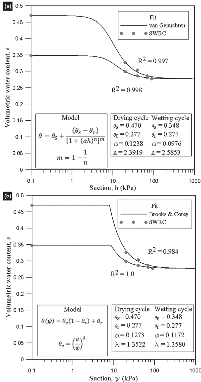
Figure 7 SWRC according to fitting models: (a) van Genuchten; (b) Brookes & Corey.
