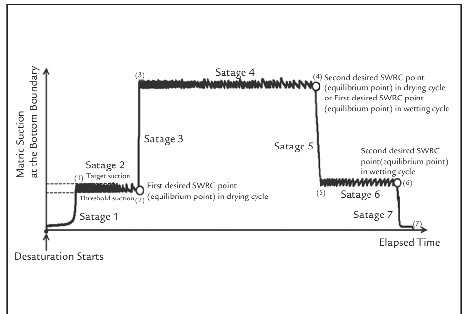
Figure 2 Schematic test results for the SWRC using the flow pump (Lee, 2011).
