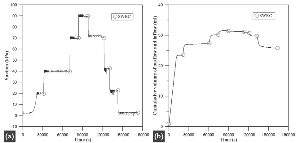
Figure 5 Test results to obtain the SWRC using the FPS.
