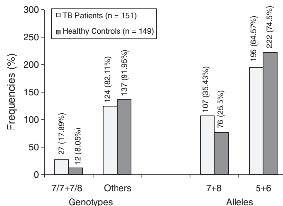
Fig. 2 – Frequencies of MIF-794CATT 5-8 genotype and allele between tuberculosis patients and healthy controls (p < 0.05).
