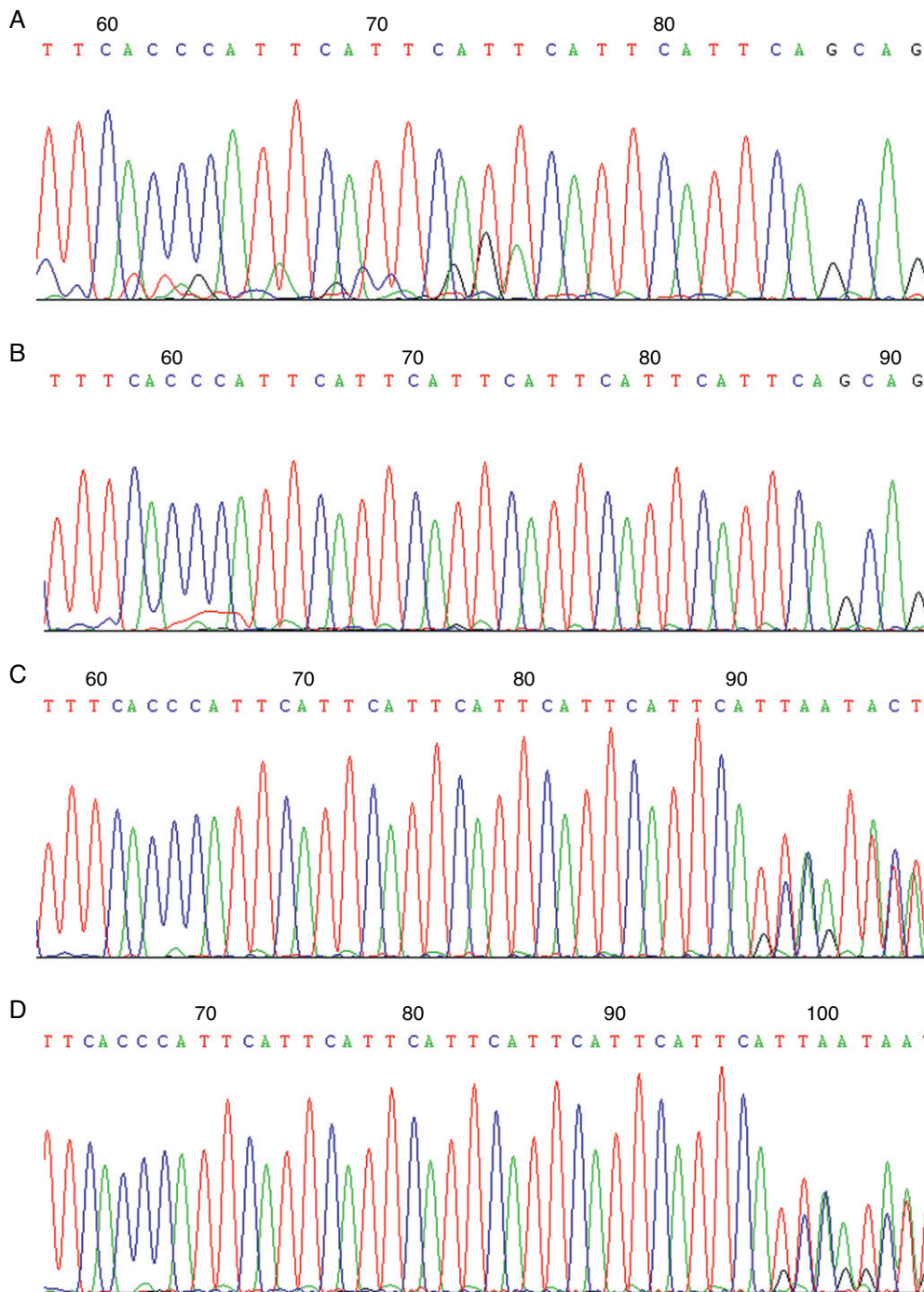
Fig. 1 – Number of the CATT sequenced repeats: A 5, B 6, C 7 and D 8.
