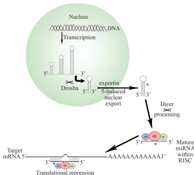
Figure 1 - The biogenesis and function of miRNAs.
