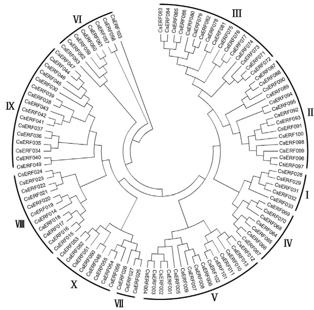
Figure S3 - Phylogenetic analysis of 103 cucumber ERF proteins. A Maximum Parsimony (MP) tree was constructed using PHYLIP3.69, by multiple sequence alignment of 103 cucumber ERF protein sequences. 10 groups are marked I to X, as described by Nakano et al. , (2006).
