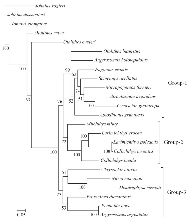
Figure 1 - Consensus trees of Sciaenidae constructed using Bayesian analysis based on P 1 partition-strategies. The accession numbers of species used in this study are flowing: Aplodinotus grunniens , EU523922; Atractoscion aequidens , DQ107824; Argyrosomus argentatus , HQ890946; Argyrosomus hololepidotus , DQ107810; Chrysochir aureus , EF607347; Collichthys lucidus , HM447239; Collichthys niveatus , NC_014263; Cynoscion guatucupa , EU074398; Dendrophysa russelii , EF607358; Johnius dussumieri , EF534120; Johnius elongates , EF534124; Johnius vogleri , EF534112; Larimichthys crocea , EU871688; Larimichthys polyactis , EU266386; Micropogonias furnieri , EU074482; Nibeia maculate , EU014249; Miichthys miuy , EU266377; Otolithes cuvieri , EF534116; Otolithes ruber , EF607450; Otolithoides biauritus , EF536890; Pogonias cromis , EU074550; Protonibeia diacanthus , EF528232; Pennahia anea , EF607487; Sciaenops ocellatus , EU180148.
