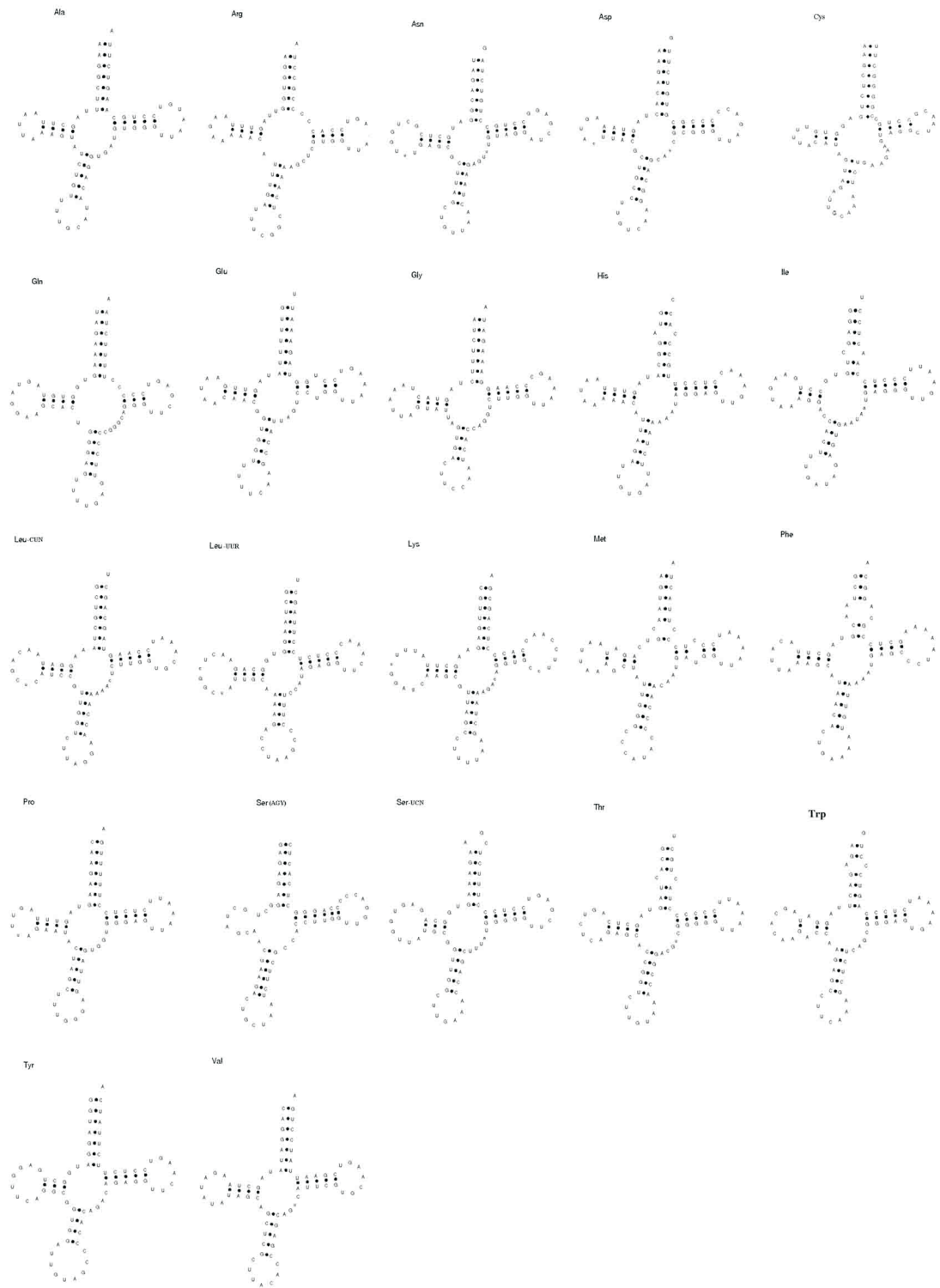
Figure S2 - Sequences of L. polyactis mitochondrial tRNA genes, represented in the clover-leaf form.
