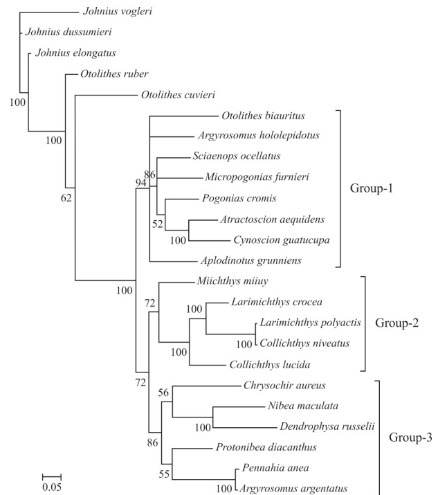
Figure 2 - Consensus trees of Sciaenidae constructed using Bayesian analysis based on P 2 partition-strategies. The accession numbers of species are those listed in Figure 1.
