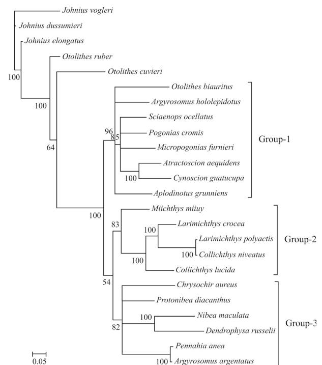
Figure 3 - Consensus trees of Sciaenidae constructed using Bayesian analysis based on P 3 partition-strategies. The accession numbers of species are those listed in Figure 1.
