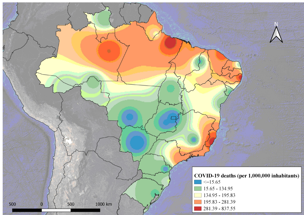
Figure 1. Cumulative rates of COVID-19 deaths in states of Brazil (per 1,000,000 inhabitants) since the first case described in March 17 th , 2020 until May 15 th , 2020.
