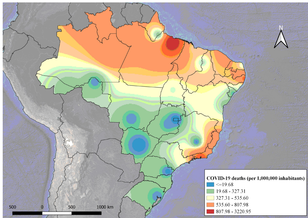
Figure 2. Mapping of cumulative rates of COVID-19 deaths in states of Brazil (per 1,000,000 inhabitants) according to Boltzmann's function forecast to June 15 th , 2020.
