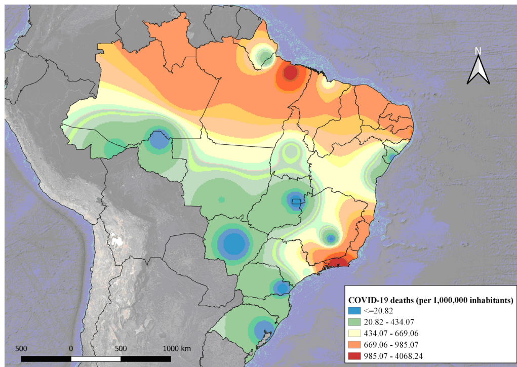
Figure 3. Mapping of cumulative rates of COVID-19 deaths in states of Brazil (per 1,000,000 inhabitants) according to Boltzmann's function forecast to July 15 th , 2020.
