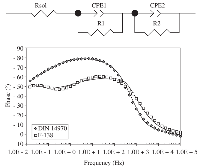
Figure 3. Equivalent circuit used to fit the impedance data for ASTM F-138 and DIN W. Nr. 1.4970 in PBS solution at room temperature.
