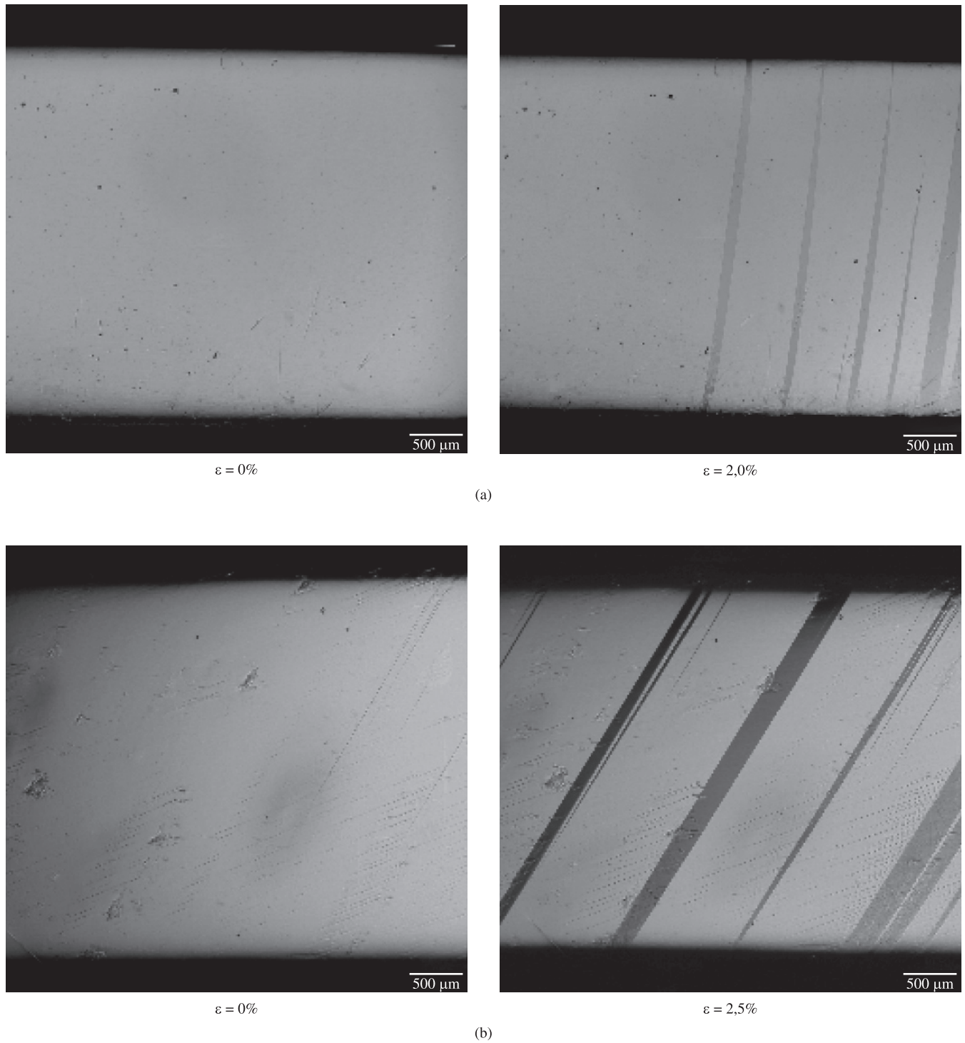
Figure 8. Micrographs of variant induced by stress (martensite plates) with different tensile axis in Cu-Al-Be tensile samples: a) CAB12b – 0 and 2%; b) CAB12c – 0 and 2.5%.
