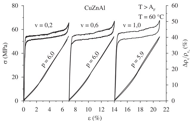
Figure 3. Strain rate influence in the superelastic electro-mechanical curves of CZA11 sample for strain rates: 0.2, 0.6 and 1.0\%/min .
