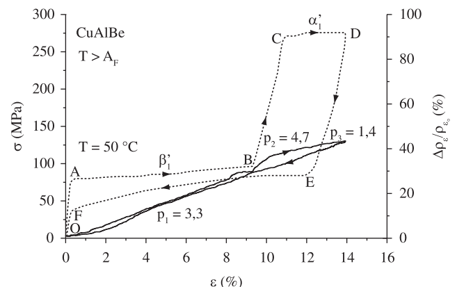
Figure 4. Electro-mechanical curves of successive martensitic transformation in the CAB5 sample.
