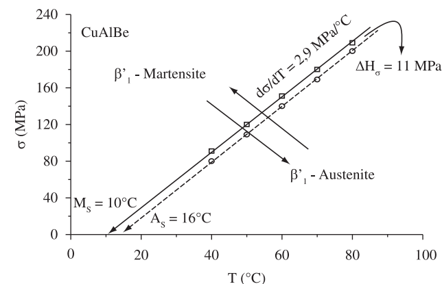
Figure 2. Phase diagram of \sigma - T type for CAB10 sample (full and dot line – direct and reverse transformation, respectively).
