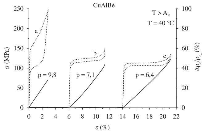
Figure 7. Superelastic tests in the CAB12 tensile samples with different crystallographic orientations (Cu-Al-Be alloy).
