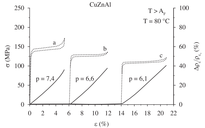
Figure 6. Superelastic tests in the CZA10 tensile samples with different crystallographic orientations (Cu-Zn-Al alloy).
