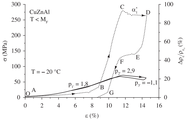
Figure 5. Electro-mechanical curves of successive martensitic transformation in the CZA3 sample.
