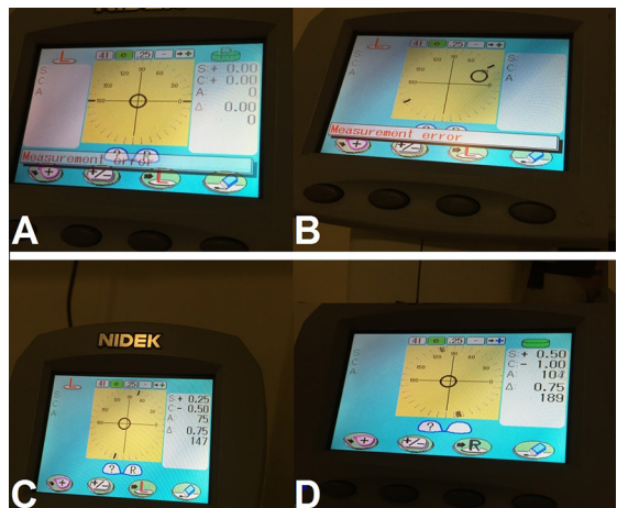
Figure 7. Measuring the membranes with the focimeter, M1 (a), M2 (b), M3 (c) e M4 (d). In the images, the angle of the focimeter display and the dark environment of the optometry clinic.
