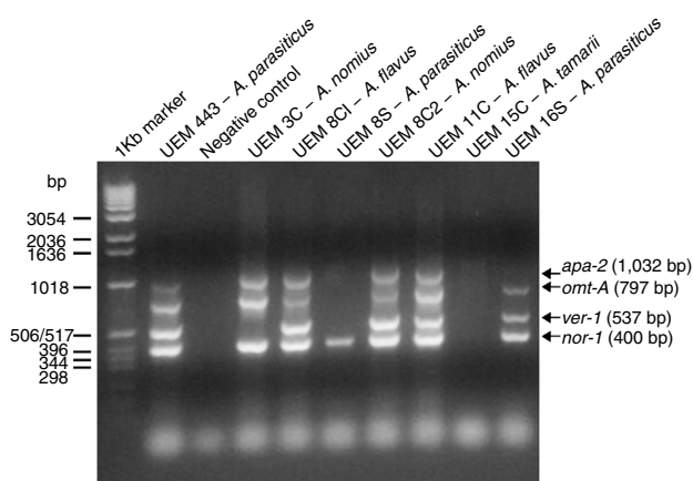
Fig. 1 – The multiplex PCR reactions. Agarose gel (1.5%) stained with ethidium bromide. 1KB marker (Thermo Fisher Scientific, USA) is the molecular marker.
