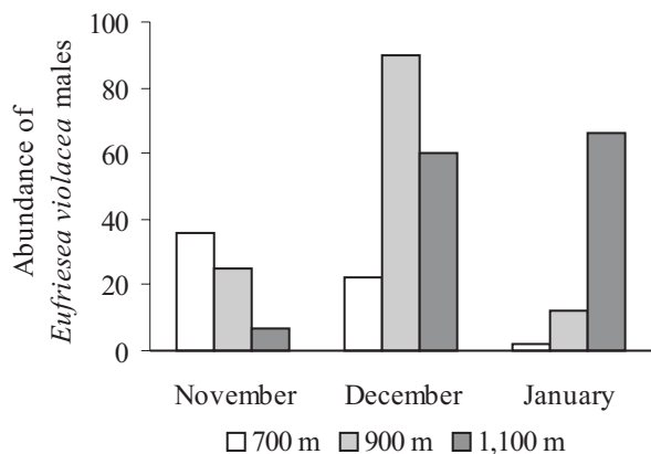
Figure 2. Monthly abundance variation of E. violacea in November and December 1998, and January 1999. Abundance differed significantly among altitudes in November ( \chi^2 = 18.91 , P < 0.001 , N = 68 ), December ( \chi^2 = 40.51 , P < 0.001 , N = 172 ) and January ( \chi^2 = 88.90 , P < 0.001 , N = 80 ).
