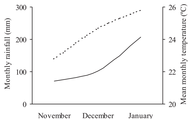
Figure 1. Mean monthly temperature (solid line) and monthly rainfall (dashed line) in November and December 1998, and January 1999 in the study site.
