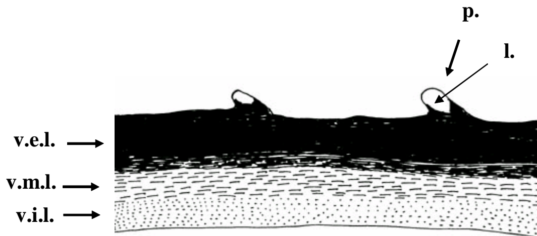
Figure 3. Transverse section of the ventral face of the egg capsule of Atlantoraja cyclophora (200X); p =prickles; l. =lumen; v.e.l. = ventral external layer; v.m.l. = ventral middle layer; v.i.l. = ventral interior layer
