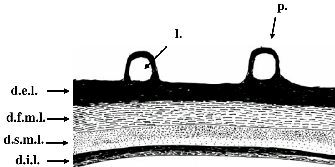
Figure 2. Transverse section of the dorsal face of the egg capsule of Atlantoraja cyclophora (200X); p =prickles; l. =lumen; d.e.l. =dorsal external layer; d.f.m.l. =dorsal first middle layer; d.s.m.l. =dorsal second middle layer; d.i.l. = dorsal interior layer.
