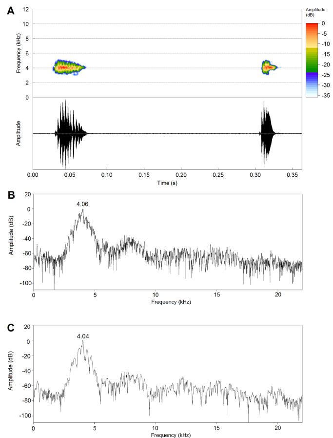
Figure 1 – Advertisement call of Dendropsophus nanus from its type locality (Resistencia, Argentina). A) Spectrogram and its respective oscillogram of the notes A and B, B) power spectrum of the note A, and C) power spectrum of the note B. Sound file: Dendrop_nanus_Resistencia_AR_1a_BFVT_Mtc.
