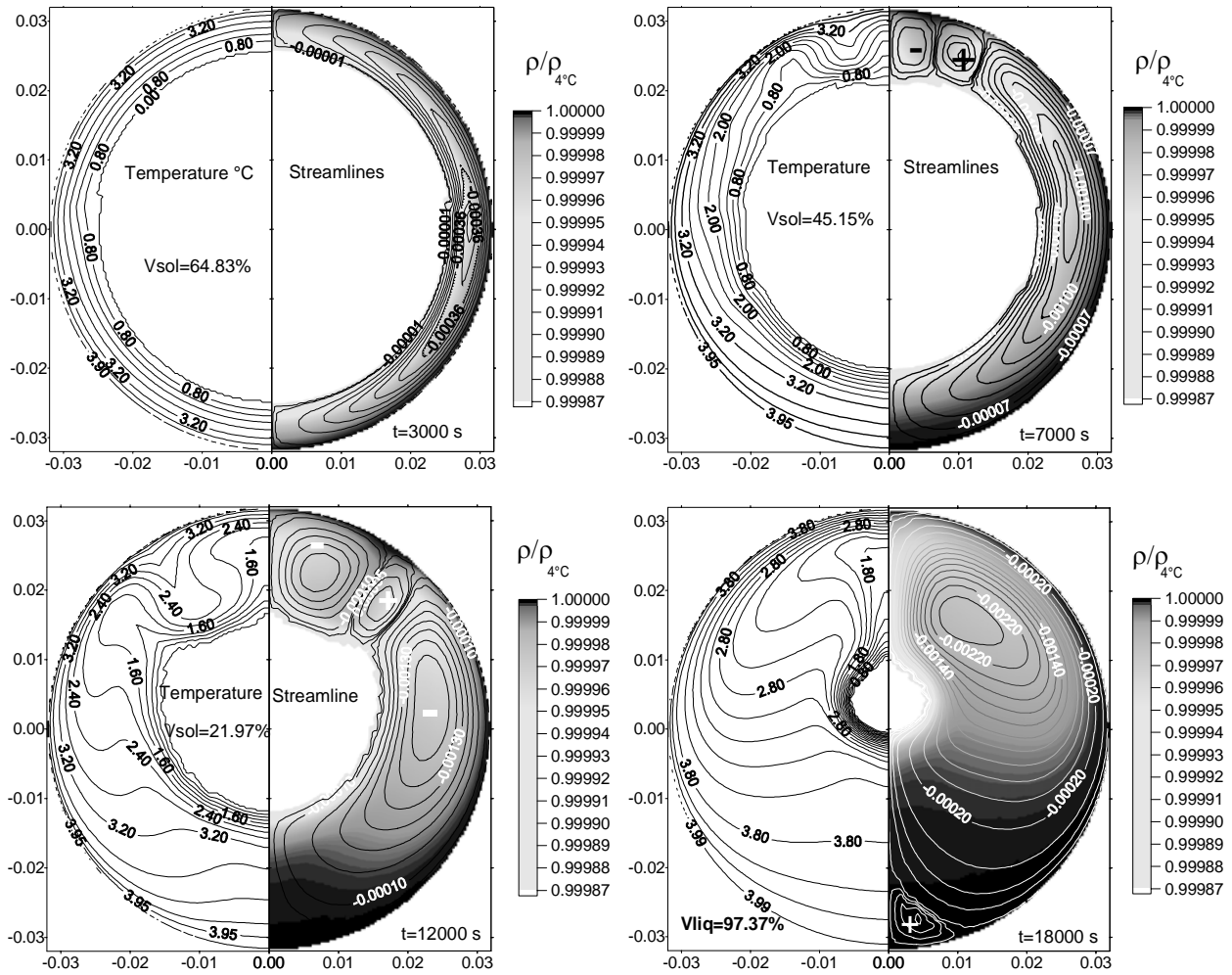
Figure 6. On the right, the streamlines (+ means anticlockwise recirculation) are juxtaposed to the density; the temperatures fields for melting with T_w = 4^\circ\text{C} , T_{ini,s} = 0^\circ\text{C} , t = 3000\text{ s} , t = 7000\text{ s} , t = 12000\text{ s} , and t = 18000\text{ s} are shown on the left.
