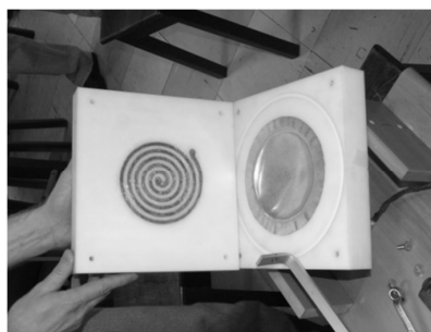
Figure 5. Die of electromagnetic forming device.
