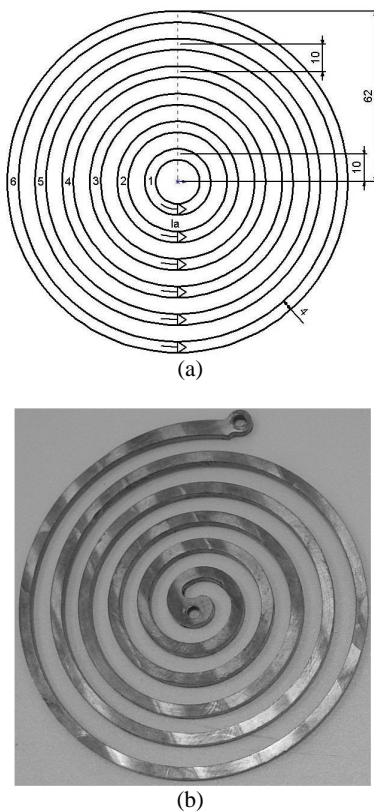
Figure 3. Flat spiral coil used in this study: (a) Simplified; (b) Real.
