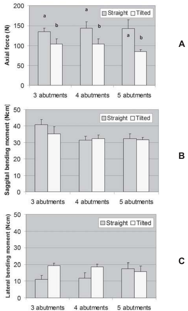
Figure 6- Axial force (A), sagittal bending moment (B), and lateral bending moment (C) in the abutment adjacent to the cantilever under loading (abutment #1). Error bars are standard error of the mean. For force values, a positive signal means compressive force and a negative signal means tensile force. Distinct letters above the bars of axial force means indicate that the means are significantly different ( \alpha=0.05 ). Sagittal and lateral bending moment means were not statistically different
