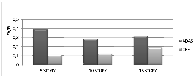
Figure 6 The effect of height of structure on (Eh/Ei) under near field records.
