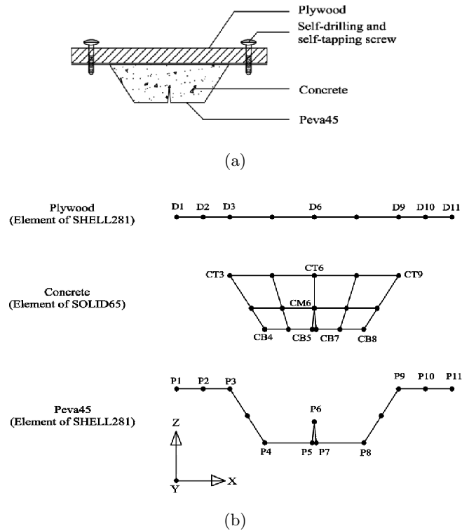
Figure 10 (a) One bay PSSDBC structural system (b) Situation of nodes in elements of one bay PSSDBC system.
