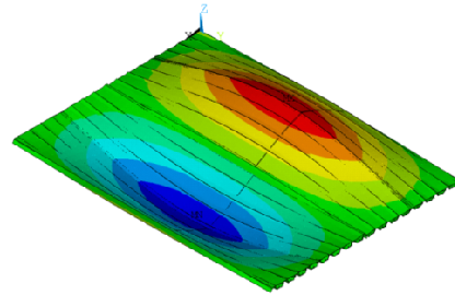
(b) Mode shape associated to the second natural frequency: f_{02}=9.208 Hz
