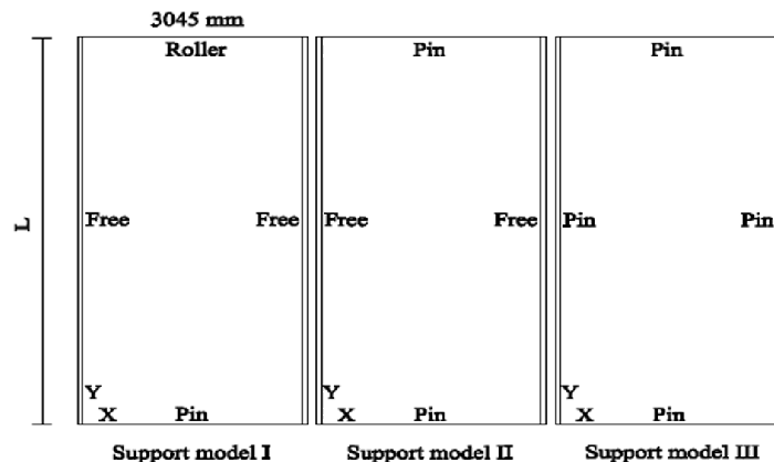
Figure 9 Considered supports in the study.
