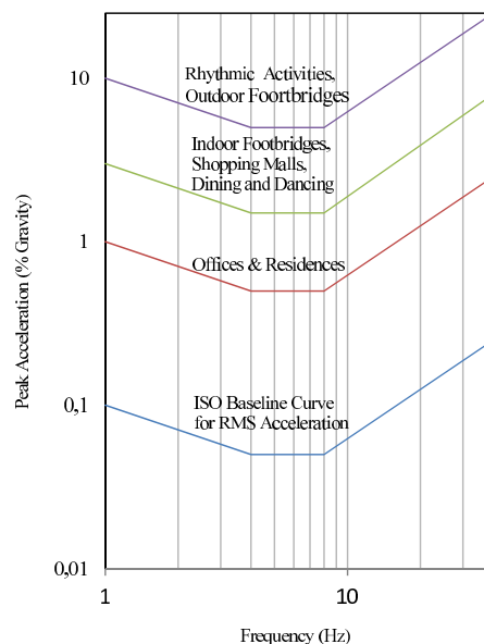
Figure 1 Recommended peak acceleration for human comfort for vibrations due to human activities [22].
