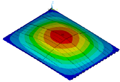
(a) Mode shape associated to the first natural frequency: f_{01}=7.326 Hz
