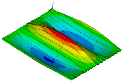
(c) Mode shape associated to the third natural frequency: f_{03}=12.385 Hz
