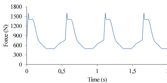
Figure 6 Fourth load model for PN9.
