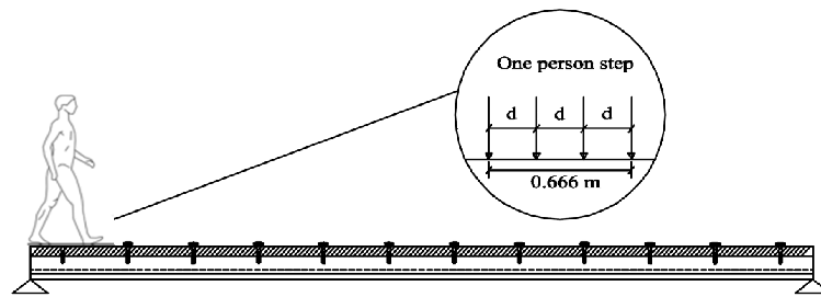
Figure 5 Person walking on the PSSDBC floor panel.
