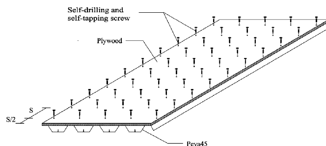
Figure 2 Profiled steel sheet dry board system.
