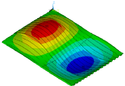
(e) Mode shape associated to the fifth natural frequency: f_{05}=19.810 Hz
