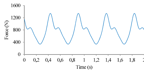
Figure 4 Second and third load models for PN9.
