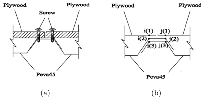
Figure 8 Detail A: (a) Constructional model (b) Analytical model
