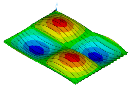
(f) Mode shape associated to the sixth natural frequency: f_{06}=22.299 Hz
