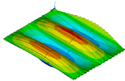
(d) Mode shape associated to the fourth natural frequency: f_{04}=18.236 Hz
