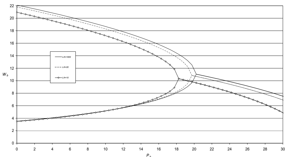
Figure 5: Variation of first and second natural frequency with respect to applied follower force for different slenderness ratios.
