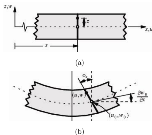
Figure 1: Cross Section of Beam in TBT; (a) before deformation; (b) after deformation (C. M. Wang, et. al, 2000).
