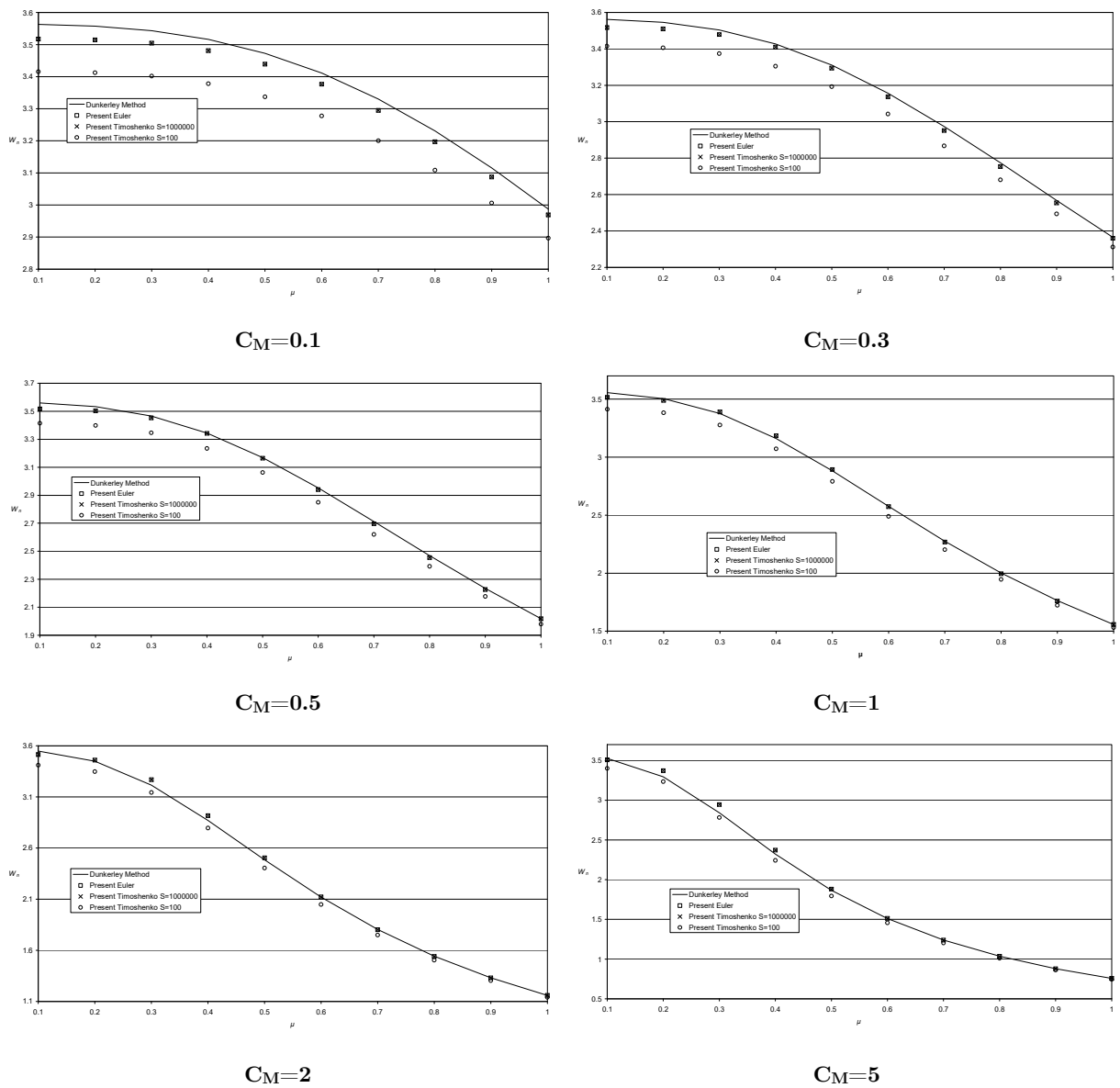
Figure 7: Effect of \mu on first natural frequency of cantilever beam with concentrated mass ( \mu=x_{CM}/L ).
