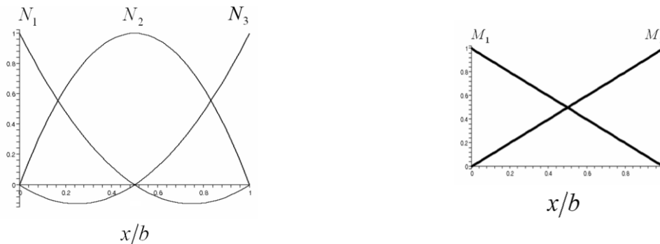
Figure 3: Linear and quadratic Lagrangian polynomials.
