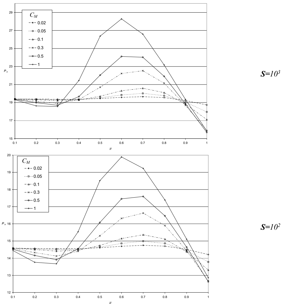
Figure 8: Critical follower force of cantilever beam for different values and locations of concentrated mass.
