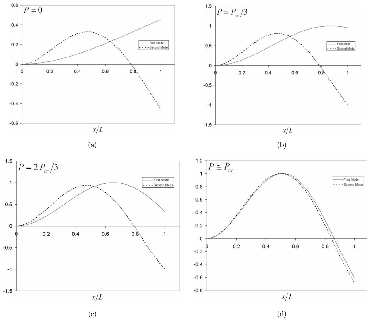
Figure 6: Mode shapes of a cantilever beam under follower force for different values of follower force.
