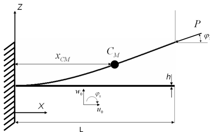
Figure 2: Geometry of cantilever beam under follower force
