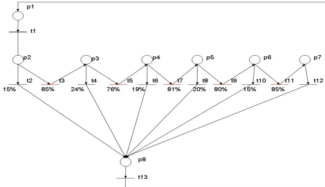
Fig. 3: Simplified model of the existing state of environmental information flows at the Regional Office
