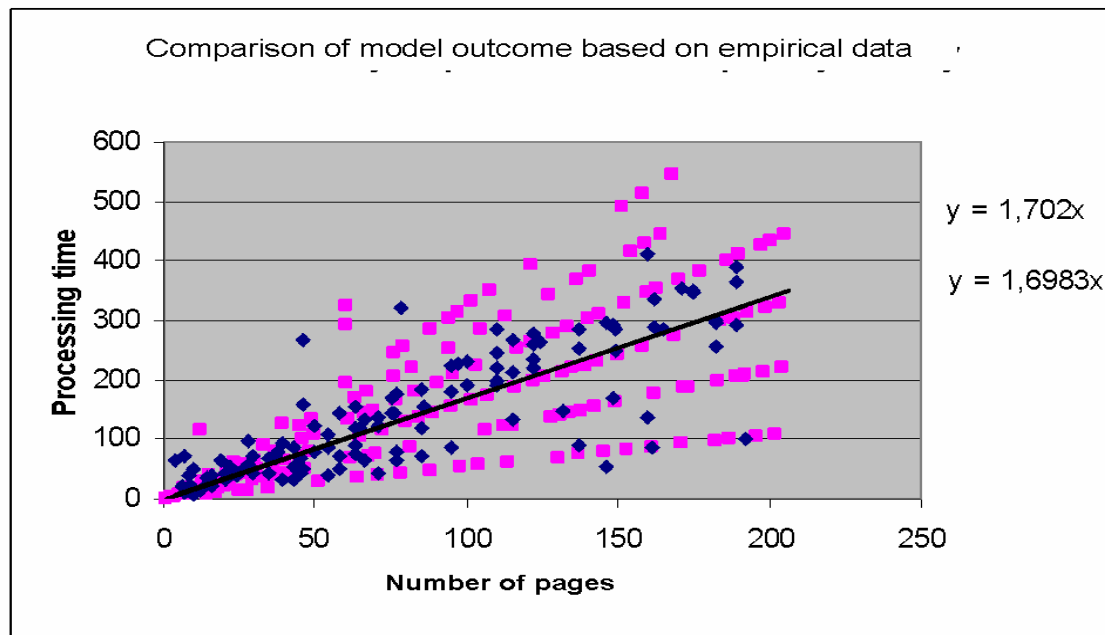
Fig. 6: Graphic comparison of model outcome in the HPSim programme based on empirical data.
