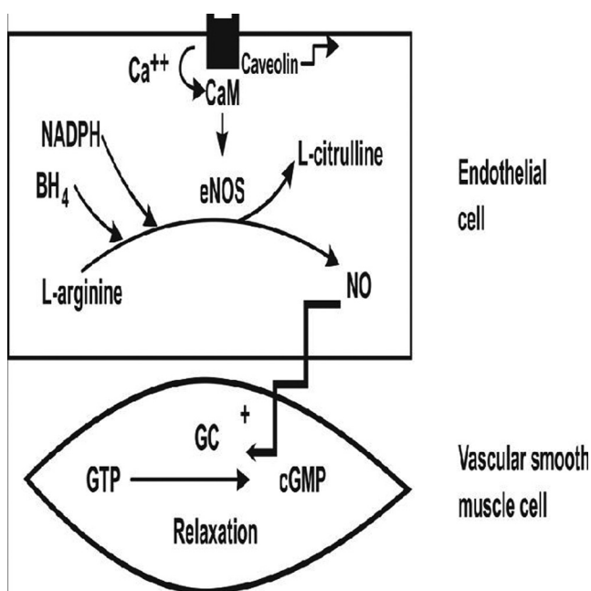
Figure 1 - Production of NO by endothelial cells. Modified from Davignon J, Ganz P. Role of endothelial dysfunction in atherosclerosis. Circulation . 2004;109 (suppl III): III27- III32. BH 4 = tetrahydrobiopterin.
