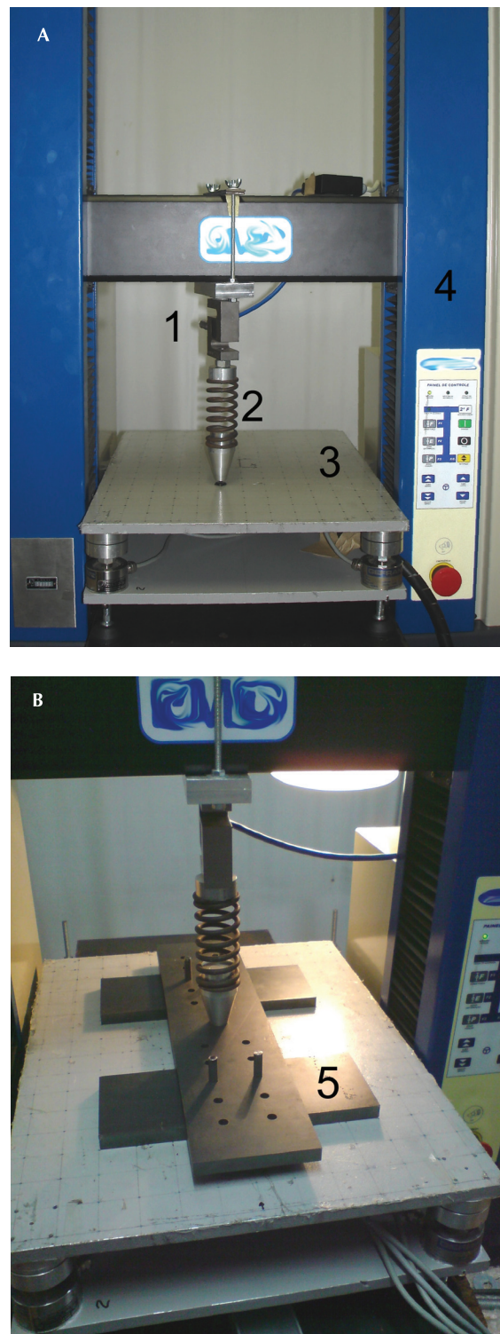
Figure 2. The stabilometric force platform was positioned in the universal testing machine to perform: A) the force threshold test that consists of the application of single point dynamic load on each position of the test grid and B) the application of distributed load; 1) load cell; 2) mechanical structure; 3) upper plate of the platform with the test grid; 4) universal testing machine; 5) two metal feet.
