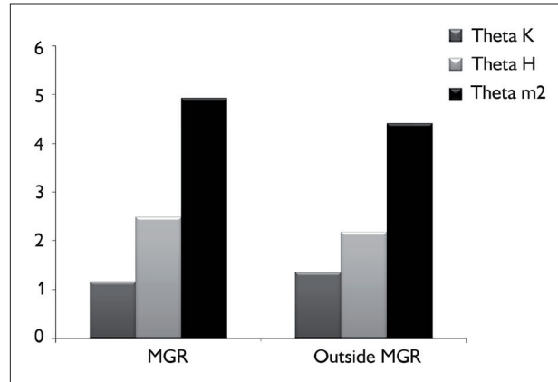
Figure 2. Theta estimators obtained from number of alleles (Theta k ), heterozygosity (Theta H ) and variance in number of repetitions (Theta m^2 ). All statistics were estimated for 11 STRs in Tupí populations from MGR (Zoró, Gavião, Suruí) and outside MGR (Ache, Urubú-Kaapor, Awá-Guajá, Wayampi, Zoé, Guarani, Parakanã). Source: Ewerton 2011.
