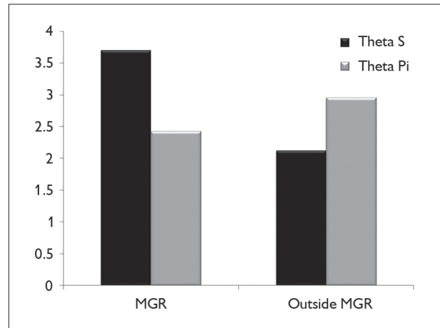
Figure 3. Theta estimators obtained from number polymorphic sites (Theta S) and Pi (Theta Pi). All statistics were estimated for haplogroup D mtDNA sequences in Tupi populations from MGR (Zoró, Gavião, Suruí) and outside MGR (Mundurukú, Asuriní do Trocará, Asuriní do Coatinemo, Araweté, Urubú-Kaapor, Parakanã, Awá-Guajá, Wayampi, Zoé; Ache; Guarani). Source: Ewerton, 2011.
