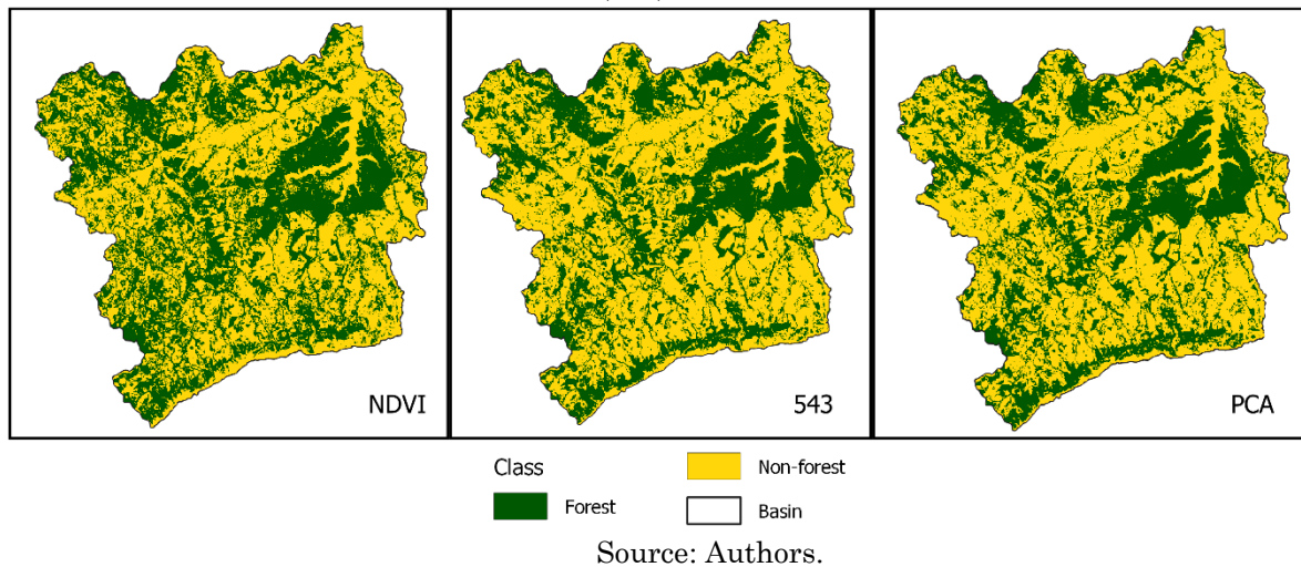
Figure 4 – Result of image classification carried out by different techniques, namely NDVI, infrared bands (543) and PCA.
