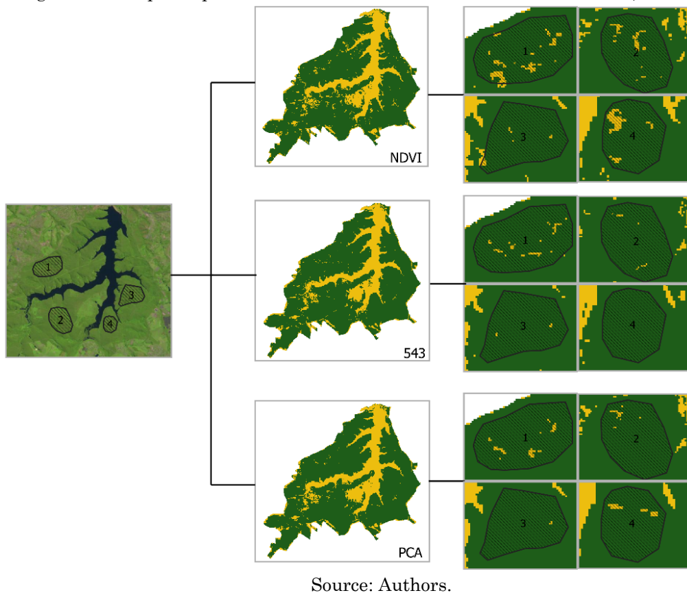
Figure 5 – Examples of variation in results of the classification of land use by different methods in some regions of the special protection area in the Serra Azul stream sub-basin, MG.
