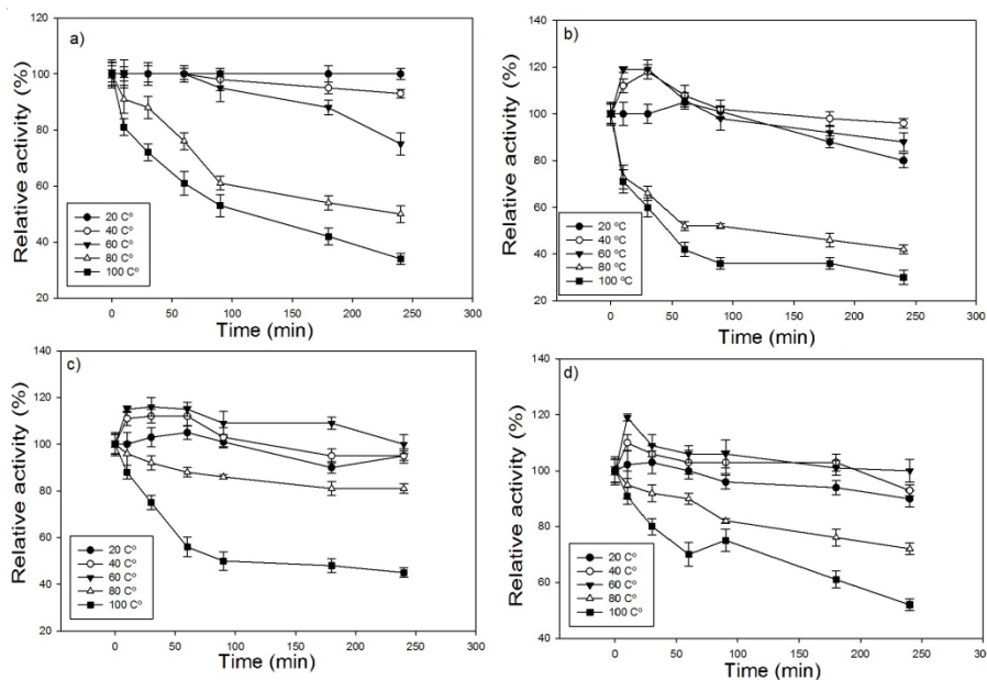
Figure 3. Thermostability of the enzymes (A) Endoglucanase, (B) total cellulases extracted of Aspergillus niger and (C) Endoglucanase, (D) total cellulases extracted Rhizopus sp.
