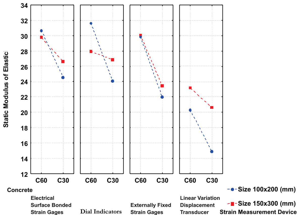
Figure 6 – Static modulus of elasticity versus specimen size, type of concrete and strain measurement device
