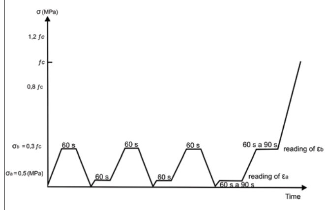
Figure 3 – Loading history for determining the modulus of elasticity – Method A (ABNT NBR 8522:2008)
