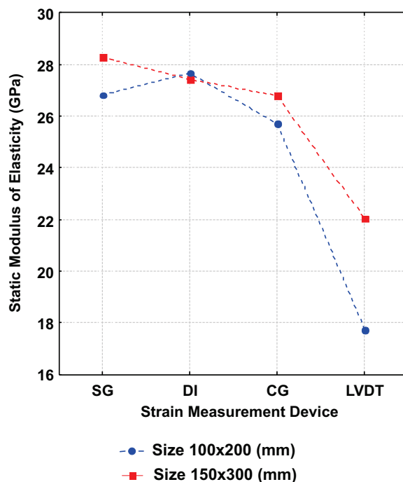
Figure 8 – Modulus of elasticity versus strain measurement device and specimen size (SG – strain gage, DI - dial indicator, CG - clip gage and LVDT)
