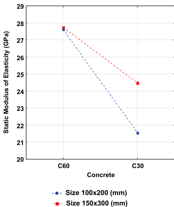
Figure 7 – Modulus of elasticity versus concrete type and specimen size (includes all measuring devices)
