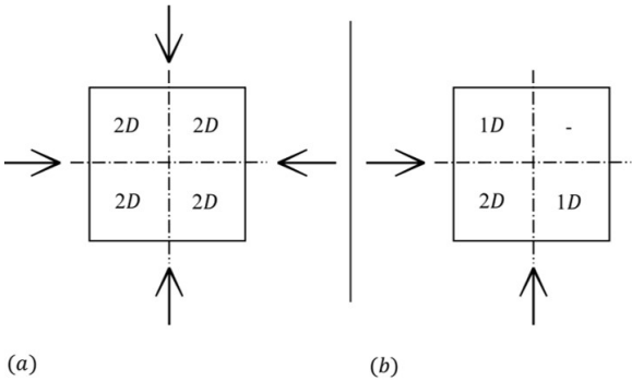
Figure 2. Distribution of temperatures in the sections with their faces exposed to fire.
