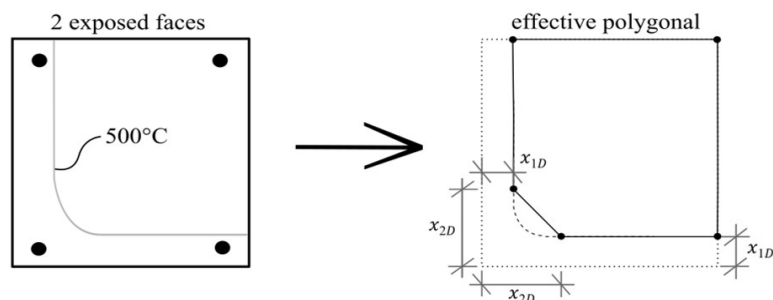
Figure 4. Approximation for the 500°C isotherm by a polygon when two faces are exposed.
