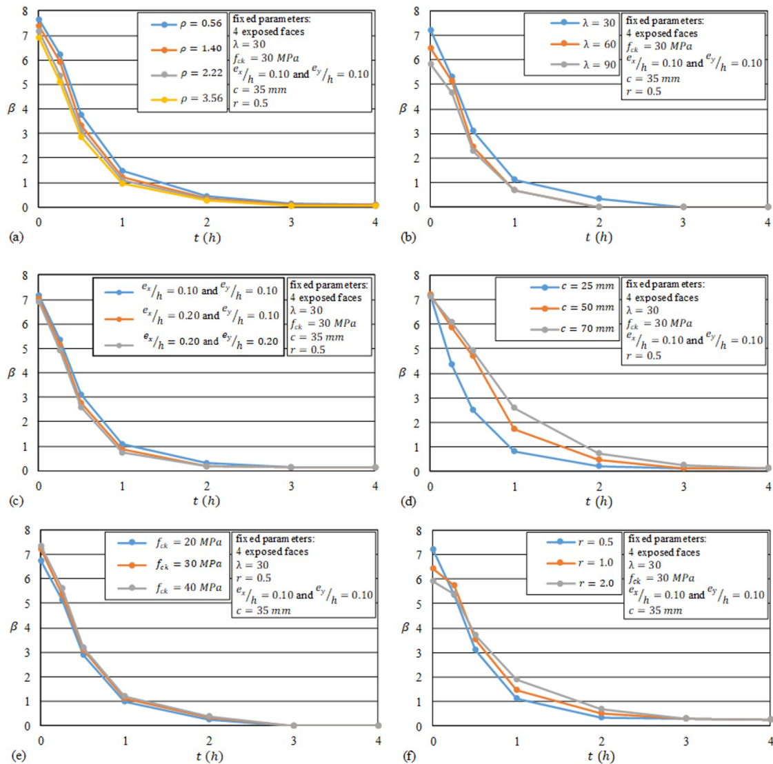
Figure 10. Parametric analyses of columns with 4 faces exposed to fire.
