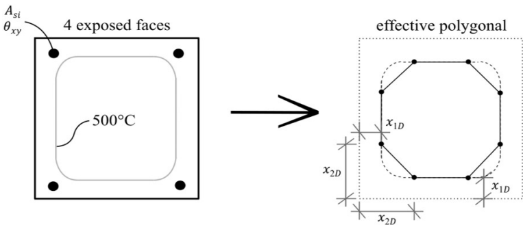
Figure 3. Approximation for the 500°C isotherm by a polygon when four faces are exposed.
