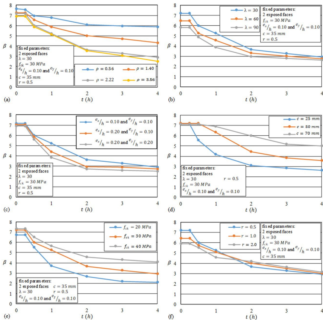
Figure 9. Parametric analyses of columns with 2 faces exposed to fire.
