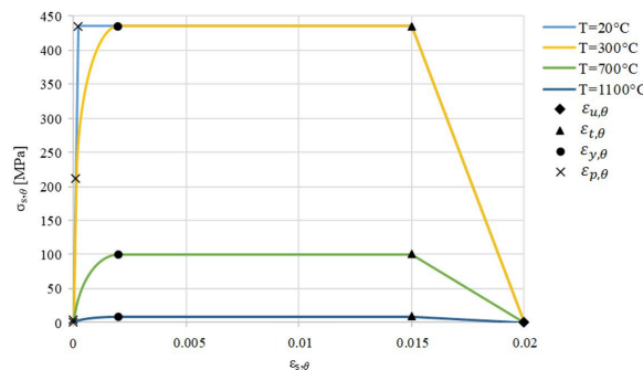
Figure 6. Steel multilinear constitutive relations as a function of temperature.
