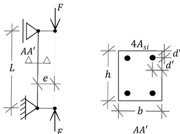
Figure 8. Geometry and boundary conditions for the studied columns.
