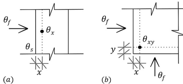
Figure 1. One and two-dimensional heat flows in concrete sections.
