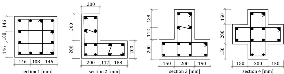
Figure 7. Column sections used for validation (dimensions not in scale).
