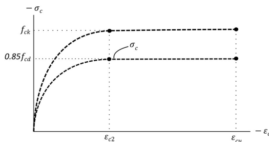
Figure 5. Idealized parabola-rectangle stress-strain diagram for concrete.
