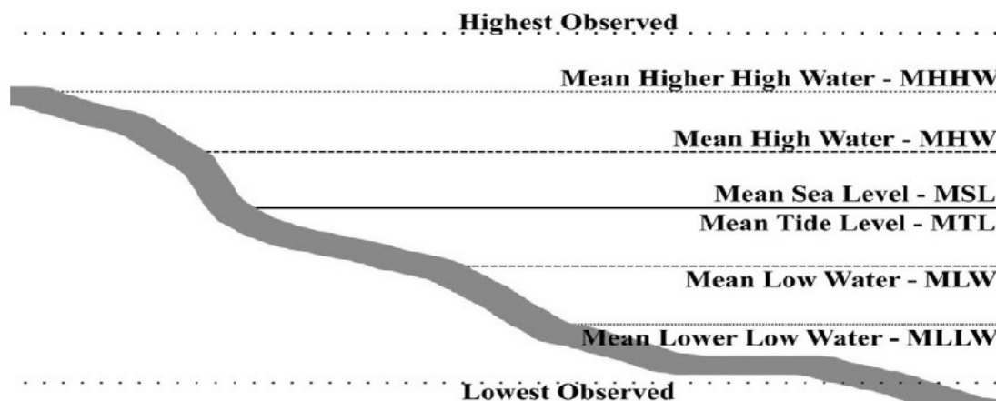
Figure 4 - Diagram of the tide datum.
