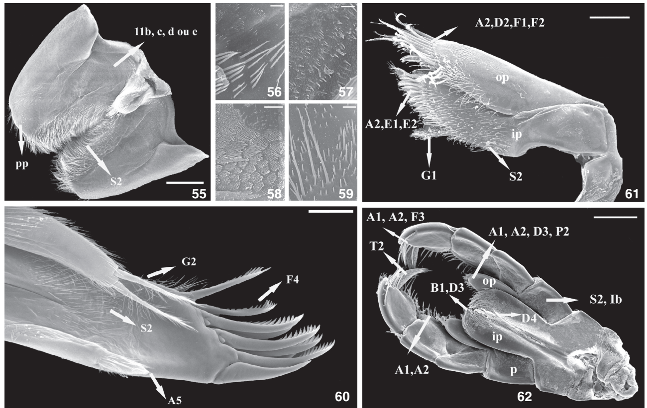
Figures 55-62. Distribution of cuticular structures on mouthparts of Hyaella : (55) lower lip, ventral view; (56-59) details of different types of decoration found on ventral surface of lower lip; (60) maxilla 1, ventral view; (61) maxilla 2 of H. castroi , dorsal view; (62) maxillipeds, ventral view. Scale bar: 55, 61 and 62 = 100 \mu\text{m} , 56-59 = 5 \mu\text{m} ; 60 = 50 \mu\text{m} . (A-F) Setae, (S) setules, (pp) projected pores, (ip) Inner plate, (op) outer plate, (p) palp, (T) denticles, (P) pores, (l) microtrichs.
