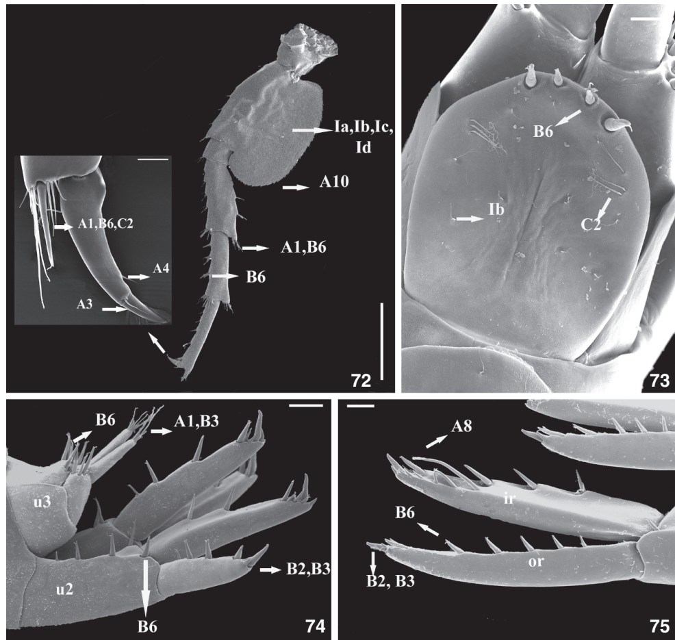
Figures 72-75. Distribution of cuticular structures on pereopods, telson and uropods of Hyalella : (72) pereopod 7, detail shows dactylus; (73) telson, dorsal view; (74) uropods 2 and 3; (75) uropod 1, male. Scale bar: 72 = 1mm; 73 = 50 \mu m; 74, 75 = 100 \mu m. (A-F) Setae, (S) setules, (T) denticles, (I) microtrichs, (ir) inner ramus, (or) outer ramus, (u1) uropod 1, (u2) uropod 2.
