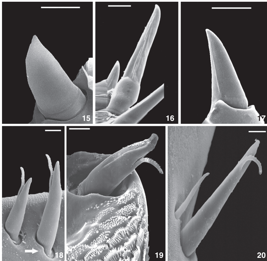
Figures 15-20. Cuspidate setae found on cuticular surface of Hyalella : (15) seta B1 from inner plate of maxillipods; (16) seta B2 from distal margin of uropod 1 (17) seta B3 from distal margin of uropod 1; (18) seta B4 from gnathopod 2 males, arrow indicates the movable socket; (19) seta B5 from lobe of gnathopod 1; (20) seta B6 from uropod 1. Scale bar = 10 \mu m.
