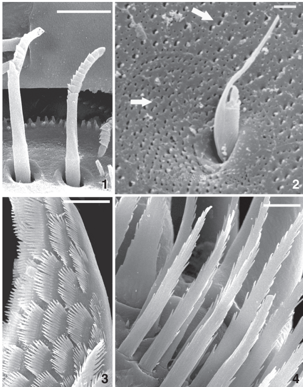
Figures 1-4. Types of cuticular structures found on Hyalella : (1) seta; (2) microtrich, arrows indicate pores; (3) denticles; (4) setules. Scale bar: a,c = 10 \mu\text{m} , d = 5 \mu\text{m} , b = 1 \mu\text{m} .
