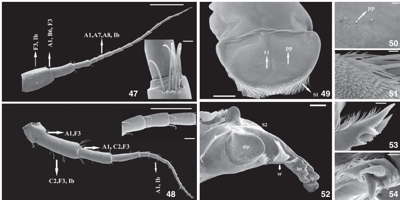
Figures 47-54. Distribution of cuticular structures of Hyalella . (47-48) From antenna 1 e 2: (47) antenna 1, detail of arrangement of setae on flagelum of antenna 1; (48) antenna 2, detail of arrangement of setae on flagelum of antenna 2; (49-54) on mouthparts: (49) upper lip, dorsal view; (50) detail of arrangement of cuticular structures on dorsal surface of upper lip; (51) detail of transition of denticles to setules on distal bord of upper lip; (52) Right mandible, arrow indicates the penicilium; (53) typical left lacinia mobilis of Hyalella ; (54) The left lacinia mobilis of H. pleoacuta could be trifurcate. Scale bar: 47-48 = 500 \mu m; 49, 52 = 50 \mu m; 50, 53 and 54 = 10 \mu m; 51 = 2 \mu m. (A-G) Setae, (S) setules, (l) microtrichs, (lm) Lacinia mobilis, (ip) incisor process, (mp) molar process, (pp) projected pores, (sr) setal row, (T) denticles.
