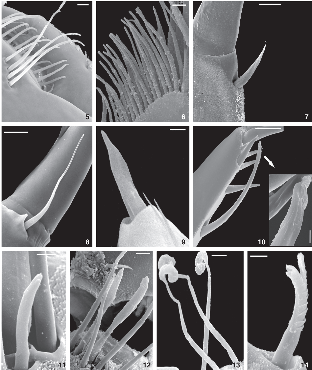
Figures 5-14. Simple setae found on cuticular surface of Hyalella : (5) seta A1 from gnathopod 1; (6) seta A2 from inner plate of maxilla 2; (7) seta A3 from dactylus of pereopods; (8) seta A4 from dactylus of pereopods; (9) seta A5 from maxilla 1; (10) seta A6 from uropod 1 from male, detail shows the distal end of the seta A6; (11) seta A7 from antenna 1; (12) seta A8 (Aesthetasc) from antenna 1; (13) seta A9 ("Curl tipped") from oostegites; (14) seta A10 from posterior margin of the coxa of pereopods. Scale bar: 5-9, 11 and 13 = 10 \mu\text{m} , 10, 12 = 5 \mu\text{m} , 14 = 2 \mu\text{m} .
