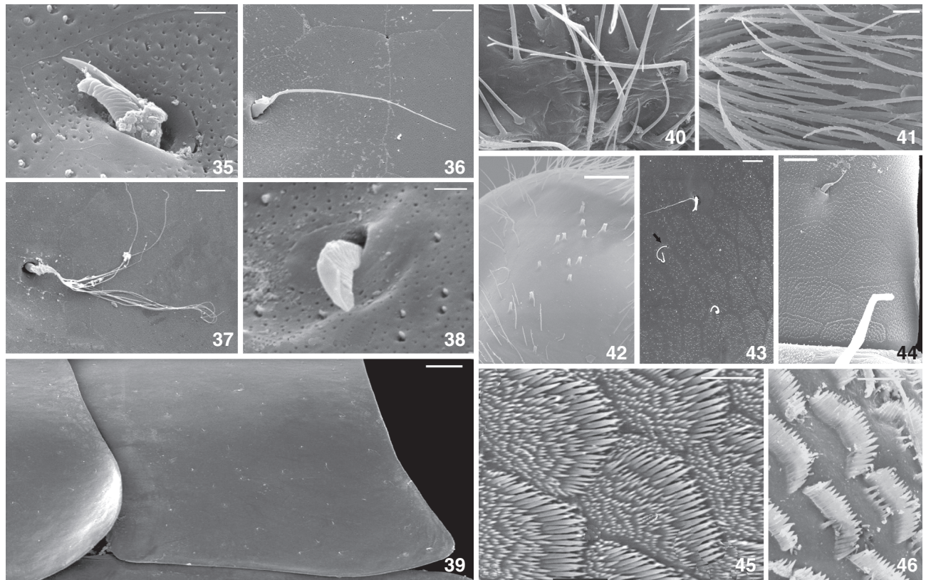
Figures 35-46. Cuticular surface of Hyalella . (35-39) Microtrichs: (35) type Ia from coxa; (36) type Ib from dorsal surface of the body; (37) type Ic from coxal plate; (38) type Id from coxal plate; (39) arrangement of microtrichs Ib on dorsal body surface; (40-46) pores and denticles: (40) setule S1 from oostegites; (41) setule S2 from maxilla 2; (42) projected pore from lower lip; (43) pores polygonal pattern P1 from telson, arrow shows some being extruded from pore; (44) pores polygonal pattern P2 from antenna 2; (46) denticles polygonal pattern T1 from gnathopod 2; (46) "comb scales" denticles T2 from posterior lobe of gnathopod 2. Scale bar: 35, 36 and 38 = 1 \mu\text{m} ; 39 = 100 \mu\text{m} ; 40 = 2 \mu\text{m} ; 37, 43, 44 and 46 = 10 \mu\text{m} ; 41 and 42 = 20 \mu\text{m} ; 45 = 5 \mu\text{m} .
