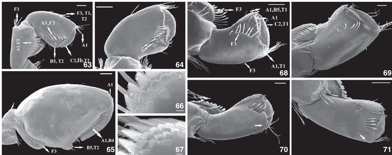
Figures 63-71. Distribution of cuticular structures on gnathopods of Hyalella . (63-67) Male: (63) gnathopod 1 of H. castroi , ventral view; (64) gnathopod 1 of H. pleoacuta , ventral view; (65) gnathopod 2 of H. castroi ; (66) detail of ornamentation of carpus of gnathopod 2 of H. castroi , ventral view; (67) detail of ornamentation of carpus of gnathopod 2 of H. pleoacuta , dorsal view; (68-71) females: (68) gnathopod 1 of H. pleoacuta , ventral view; (69) gnathopod 1 of H. castroi , ventral view; (70) gnathopod 2 of H. pleoacuta , ventral view, arrow shows "comb scales" on bordo antero distal margin; (71) gnathopod 2 of H. castroi , arrow shows the absence of "comb scales" on antero distal margin. Scale bar: 63, 64, 68 and 70 = 100 \mu m; 65 = 200 \mu m; 66 and 67 = 5 \mu m; 69 and 71 = 50 \mu m. (A-F) Setae, (S) setules, (T) denticles, (I) microtrichs, (P) pores.
