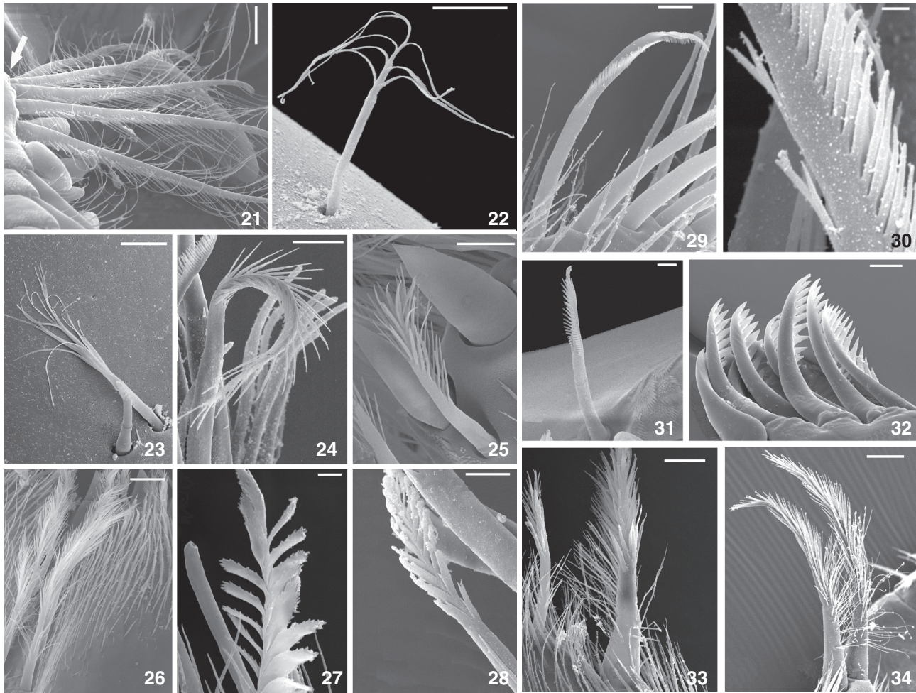
Figures 21-34. Plumose, pappose and serrulate setae found on cuticular surface of Hyalella : (21) plumose seta C1 from pleopods, arrow indicates the infracuticular articulation; (22) plumose seta C2 from telson; (23) pappose seta D1 from antenna 2; (24) pappose seta D2 from inner plate of maxilla 2; (25) pappose seta D3 from inner plate of maxillipeds; (26) pappose seta D4 from inner plate of maxillipeds; (27) serrulate seta E1 from inner plate of maxilla 2; (28) serrulate seta E2 from inner plate of maxilla 2; (29) serrate seta F1 from outer plate of maxilla 2; (30) serrate seta F2 from inner plate of maxilla 2; (31) serrate seta F3 from gnathopod 2; (32) serrated seta F4 from maxilla 1; (33) papposerrate setae G1 from inner plate of maxilla 2; (34) papposerrate setae G2 from inner plate of maxilla 1. Scale bar: 21, 26, 29, 30 and 34 = 20 \mu\text{m} ; 22-25, 31 and 33 = 10 \mu\text{m} ; 27-28 = 2 \mu\text{m} ; 32 = 1 \mu\text{m} .
